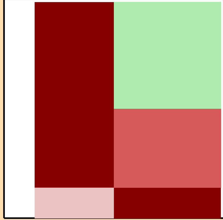
\Delta\sigma/\sigma vs. E for ^{214}\text{Pb}(n,p)
