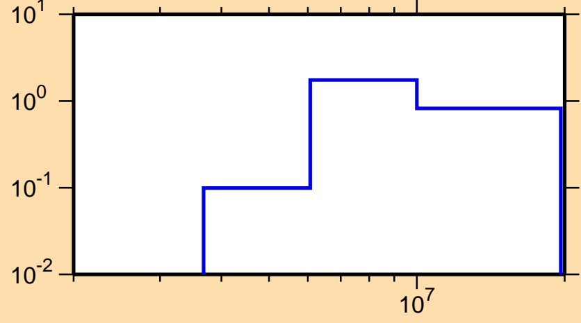
\sigma vs. E for ^{214}\text{Pb}(n,2n)
