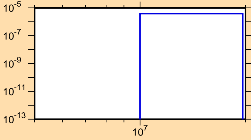
\sigma vs. E for ^{214}\text{Pb}(n,d)
