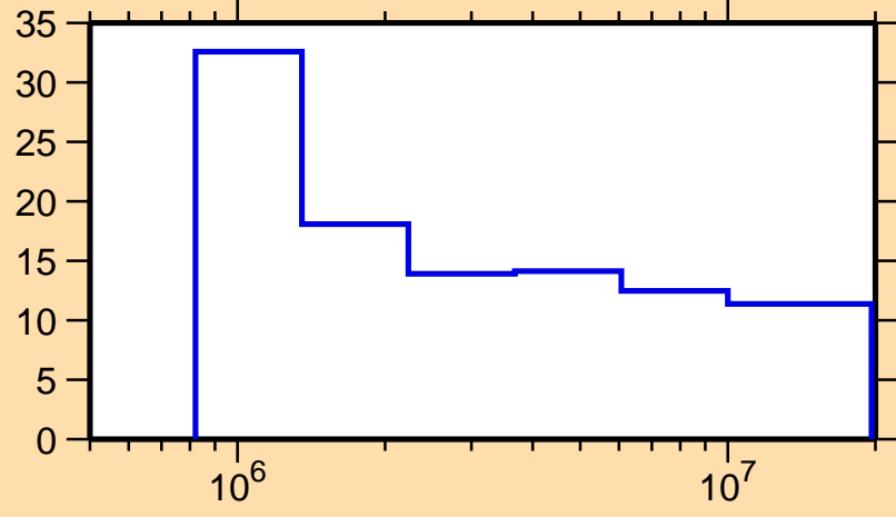
\Delta\sigma/\sigma vs. E for ^{214}\text{Pb}(n,n\text{onel.})
