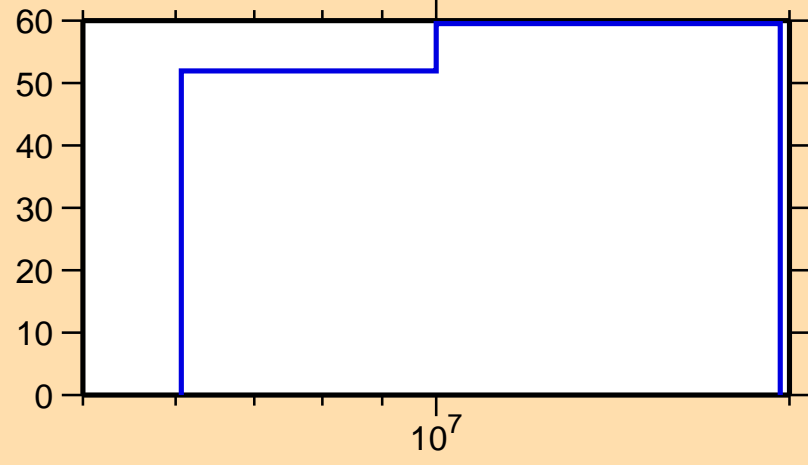
\Delta\sigma/\sigma vs. E for ^{214}\text{Pb}(n,ncont.)
