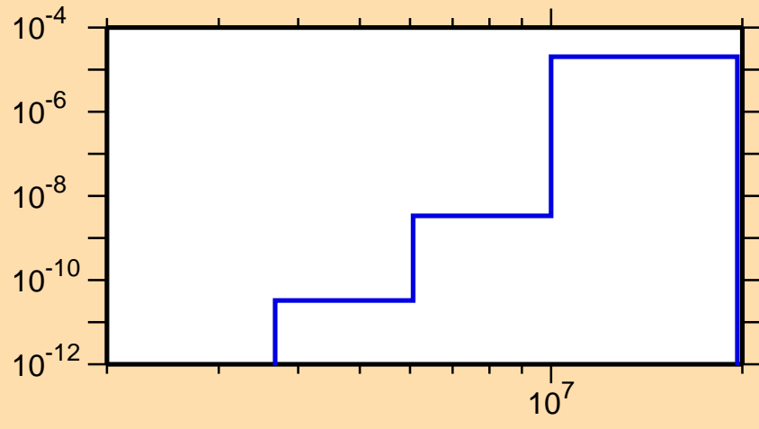
\sigma vs. E for ^{214}\text{Pb}(n,\alpha)
