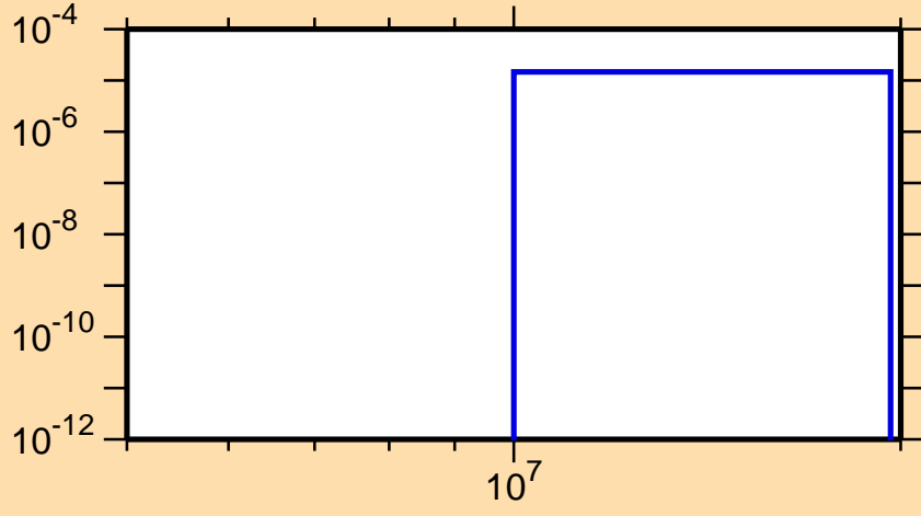
\sigma vs. E for ^{214}\text{Pb}(n,t)
