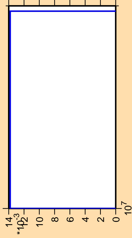
\Delta\sigma/\sigma vs. E for ^{214}\text{Pb} (mt 11)
