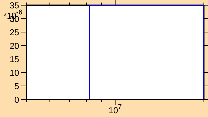
\sigma vs. E for ^{214}\text{Pb}(n,p)
