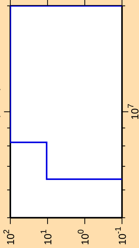
\Delta\sigma/\sigma vs. E for ^{214}\text{Pb}(n,n\alpha)
