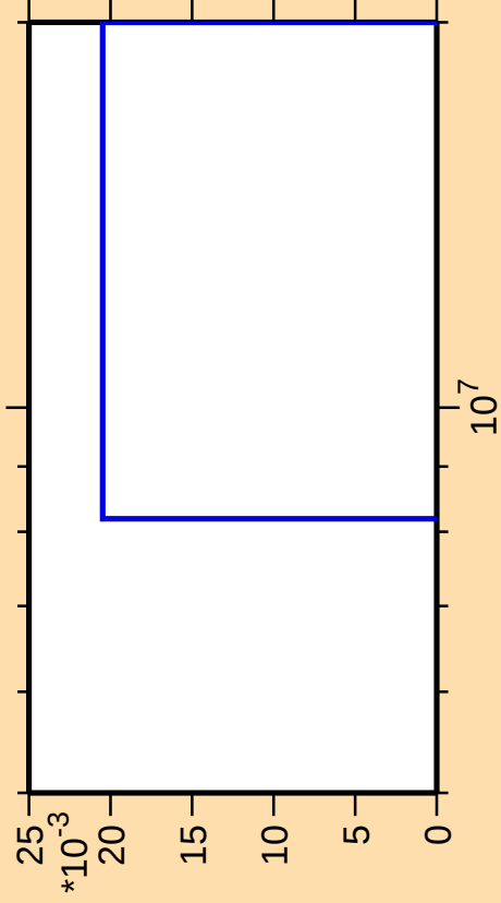
\Delta\sigma/\sigma vs. E for ^{214}\text{Pb}(\text{mt 11})
