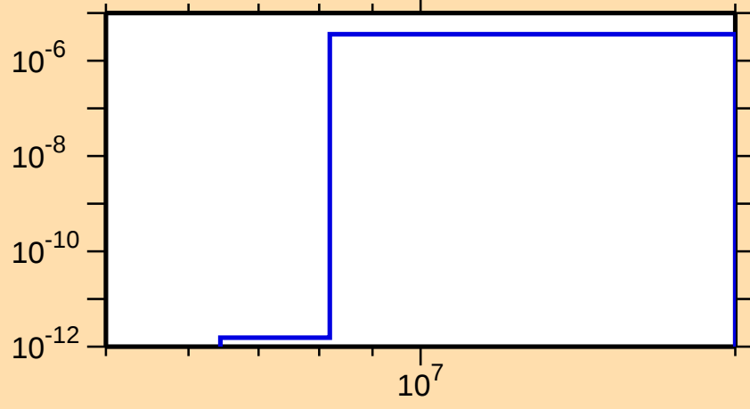
\sigma vs. E for ^{214}\text{Pb}(n,n\alpha)
