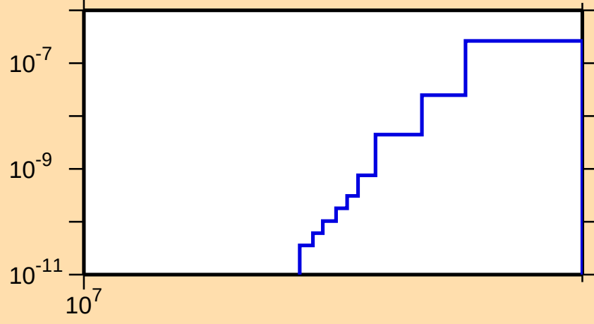
\sigma vs. E for ^{216}\text{Pb}(n,2n\alpha)
