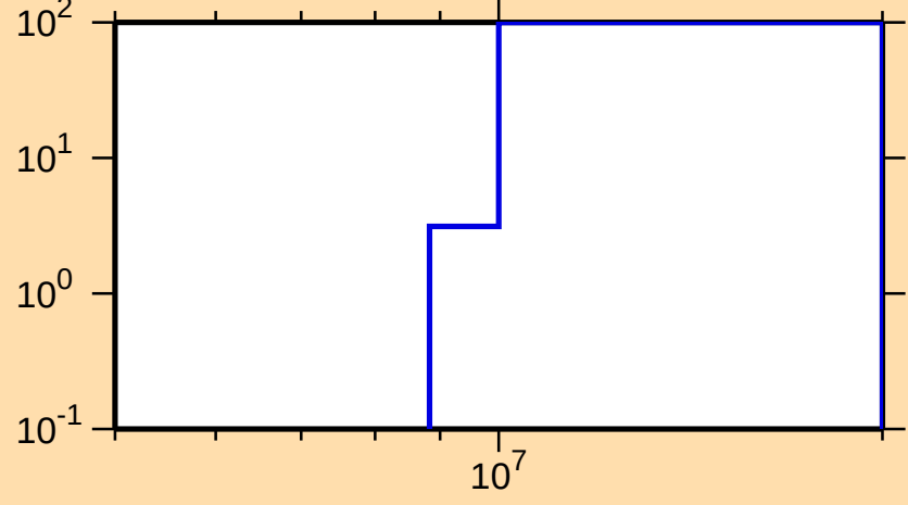
\Delta\sigma/\sigma vs. E for ^{216}\text{Pb}(n,p)
