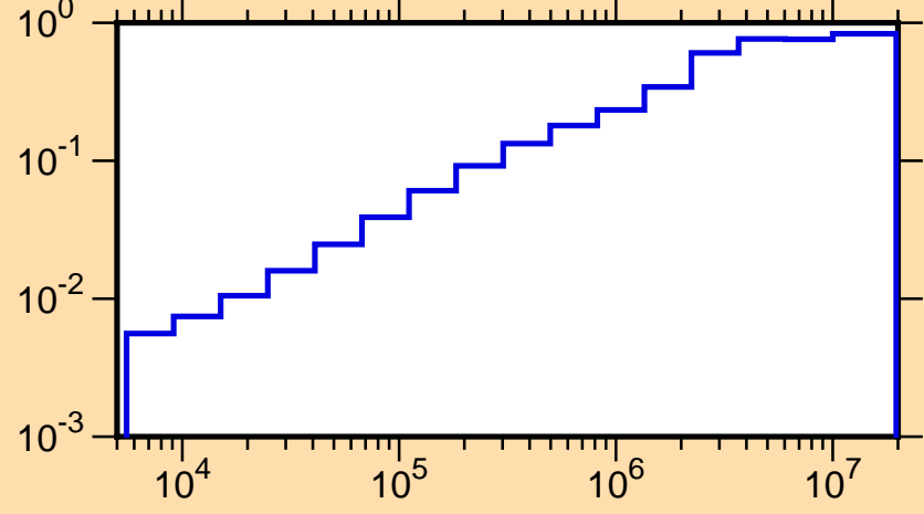
\mu vs. E for ^{216}\text{Pb}(\text{mt251})
