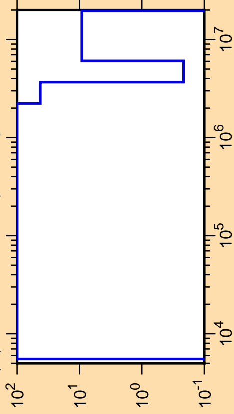
\Delta\mu/\mu vs. E for ^{216}\text{Pb}(\text{mt251})
