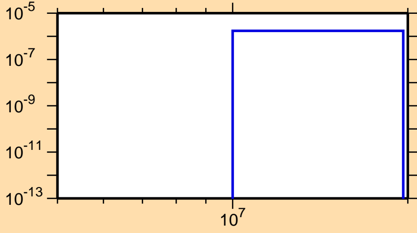
\sigma vs. E for ^{216}\text{Pb}(n,d)
