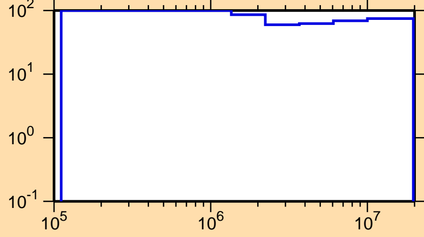
\Delta\sigma/\sigma vs. E for ^{216}\text{Pb}(n,n\text{onel.})
