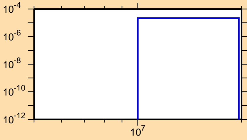
\sigma vs. E for ^{216}\text{Pb}(n,p)
