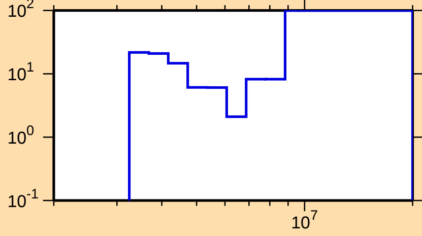
\Delta\sigma/\sigma vs. E for ^{217}\text{Pb}(n,2n)
