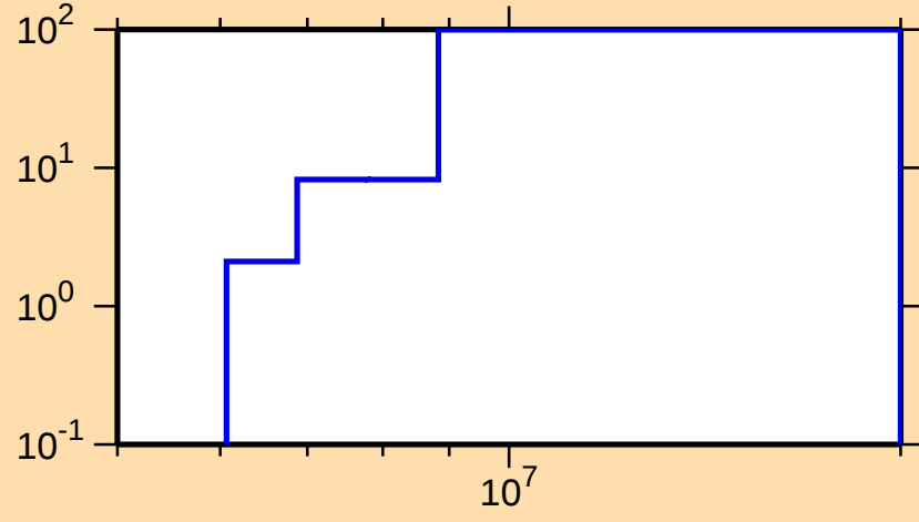
\Delta\sigma/\sigma vs. E for ^{217}\text{Pb}(n,2n)
