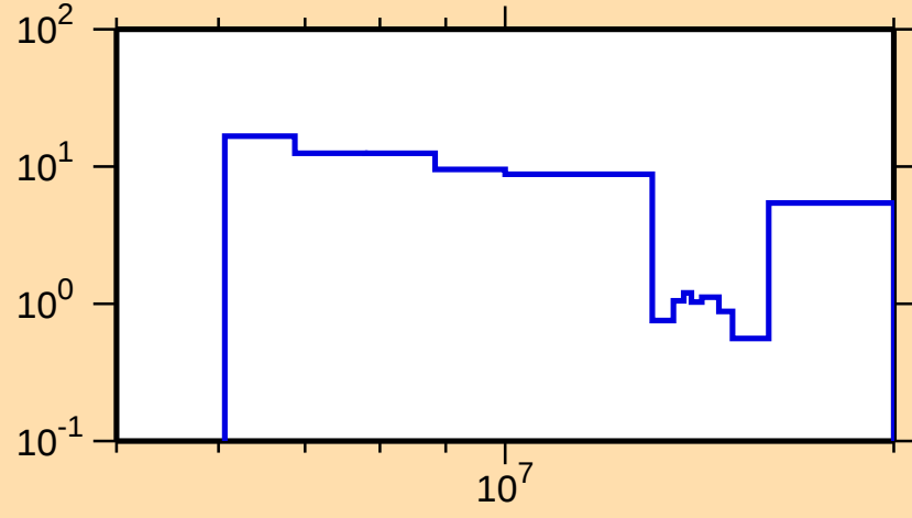
\Delta\sigma/\sigma vs. E for ^{217}\text{Pb}(n,\text{nonel.})
