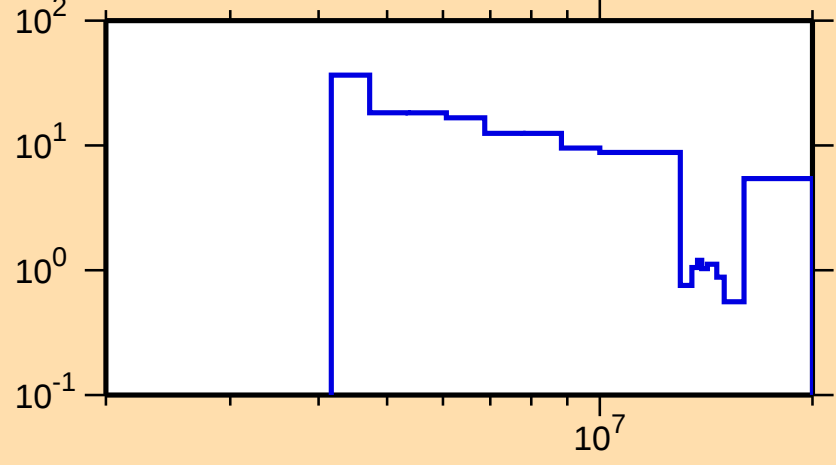
\Delta\sigma/\sigma vs. E for ^{217}\text{Pb}(n,\text{nonel.})
