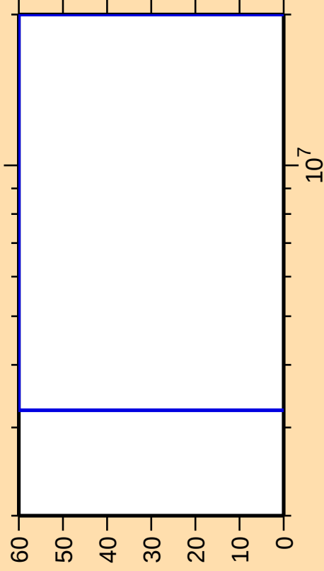
\Delta\sigma/\sigma vs. E for ^{217}\text{Pb}(n,n\text{cont.})
