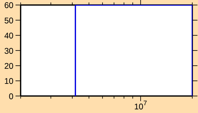
\Delta\sigma/\sigma vs. E for ^{217}\text{Pb}(n,\gamma)
