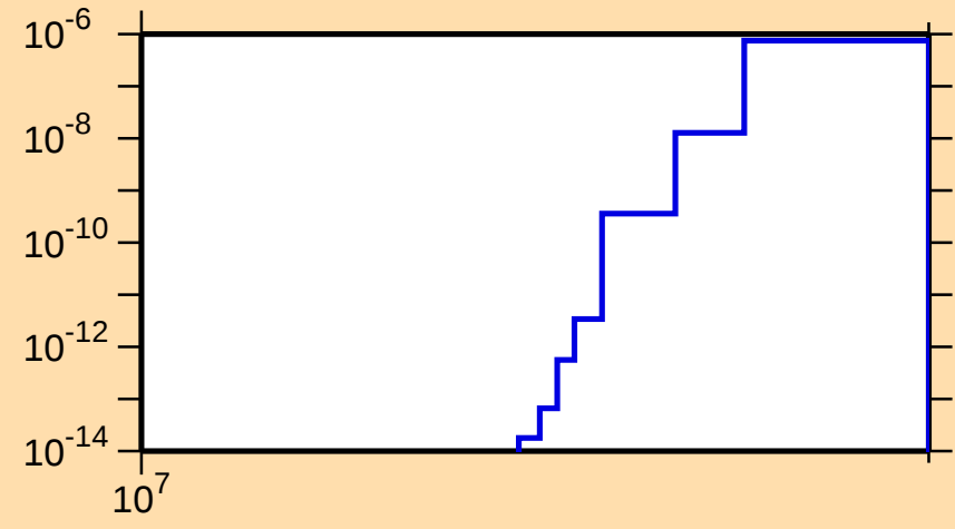
\sigma vs. E for ^{217}\text{Pb}(n,\text{nd})
