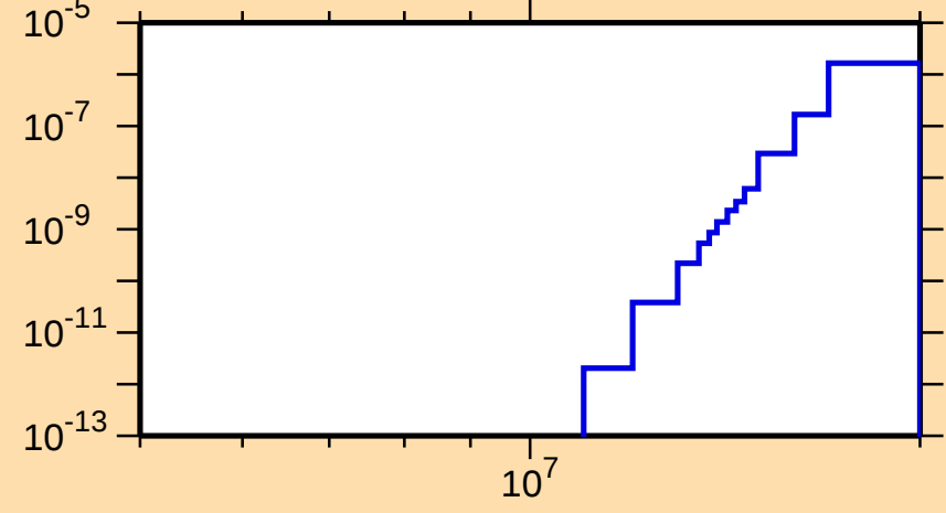
\sigma vs. E for ^{217}\text{Pb}(n,2n\alpha)
