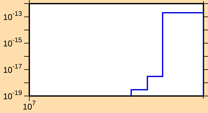
\sigma vs. E for ^{217}\text{Pb}(\text{mt 11})
