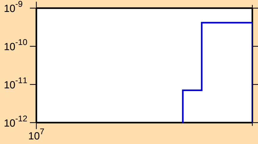
\sigma vs. E for ^{217}\text{Pb}(n,3n\alpha)
