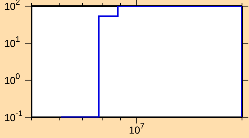
\Delta\sigma/\sigma vs. E for ^{217}\text{Pb}(n,p)
