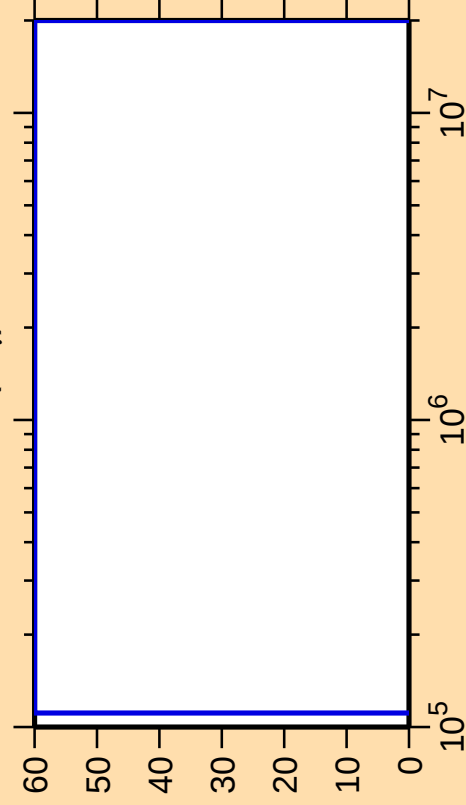
\Delta\sigma/\sigma vs. E for ^{217}\text{Pb}(n,\gamma)
