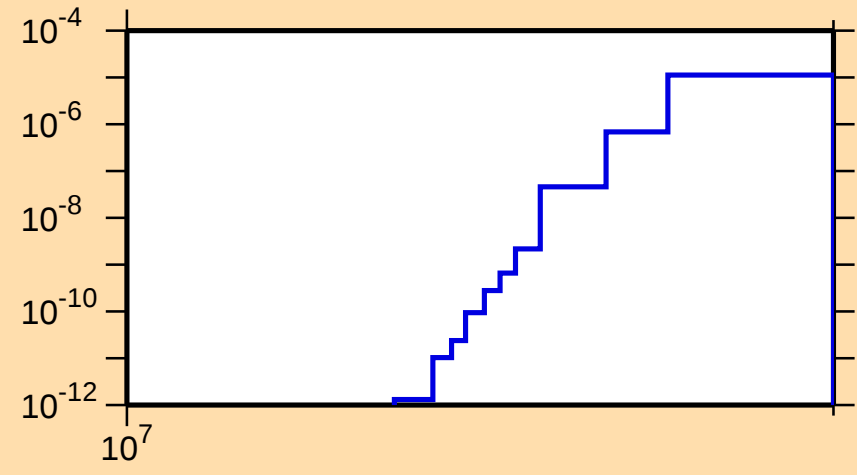
\sigma vs. E for ^{217}\text{Pb}(n,\text{nt})
