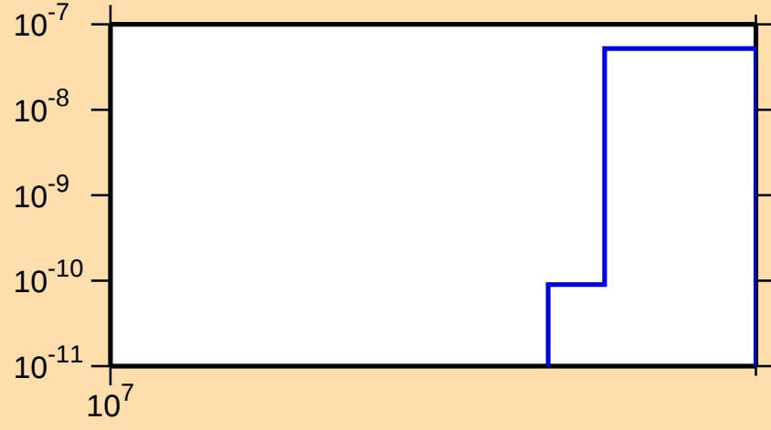
\sigma vs. E for ^{217}\text{Pb}(n,2np)
