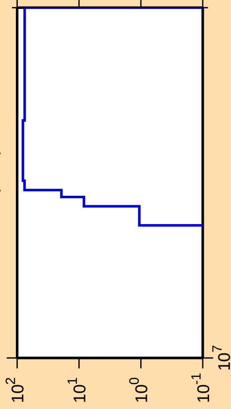
\Delta\sigma/\sigma vs. E for ^{217}\text{Pb}(n,\text{nt})
