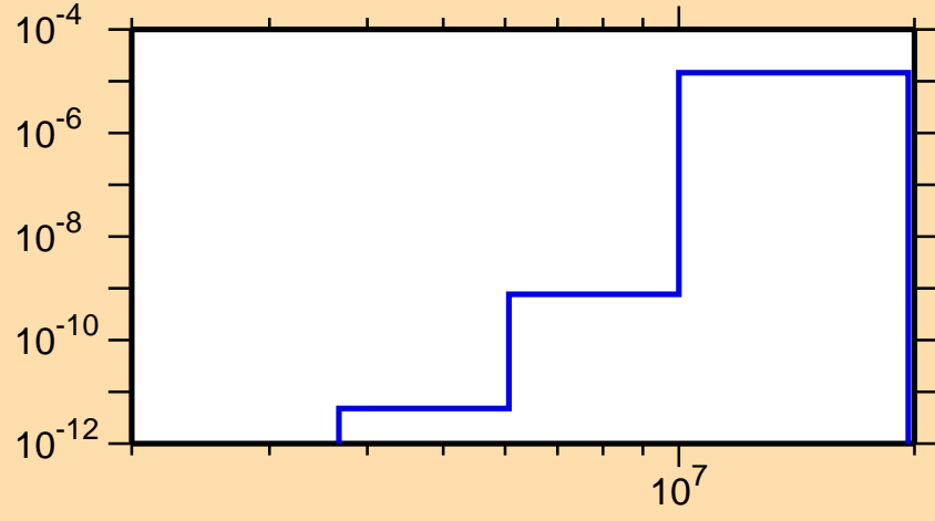
\sigma vs. E for ^{217}\text{Pb}(n,\alpha)
