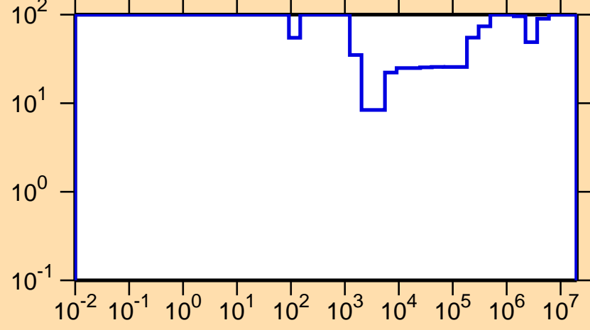
\Delta\sigma/\sigma vs. E for ^{217}\text{Pb}(n,\text{el.})
