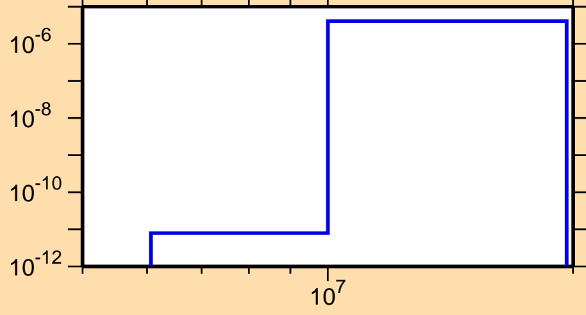
\sigma vs. E for ^{217}\text{Pb}(n,n\alpha)
