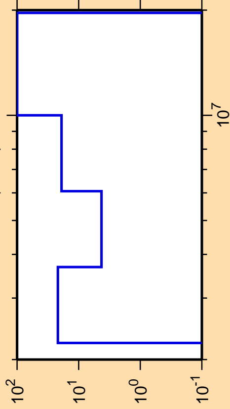
\Delta\sigma/\sigma vs. E for ^{217}\text{Pb}(n,2n)
