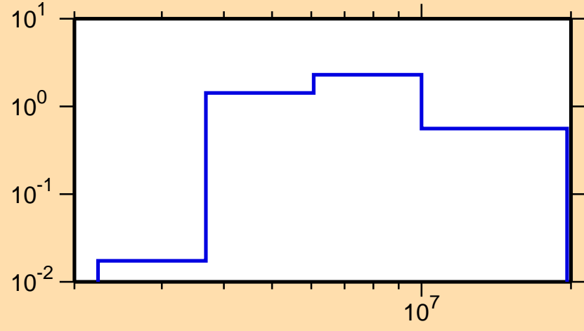
\sigma vs. E for ^{217}\text{Pb}(n,2n)
