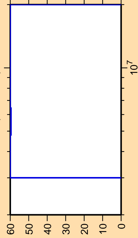
\Delta\sigma/\sigma vs. E for ^{98}\text{Pd}(n,\text{ncont.})
