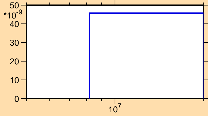
\sigma vs. E for ^{98}\text{Pd}(n,2np)
