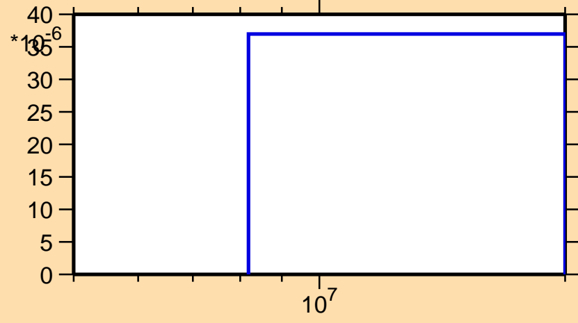
\sigma vs. E for ^{98}\text{Pd}(n,t)
