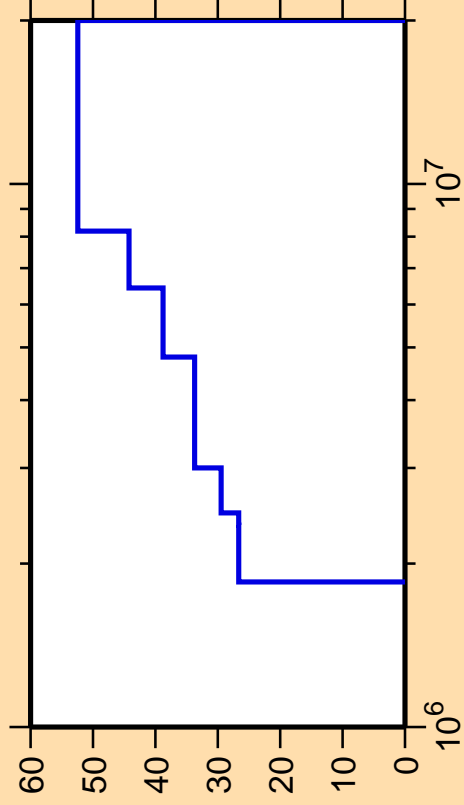
\Delta\sigma/\sigma vs. E for ^{98}\text{Pd}(n,n_3)
