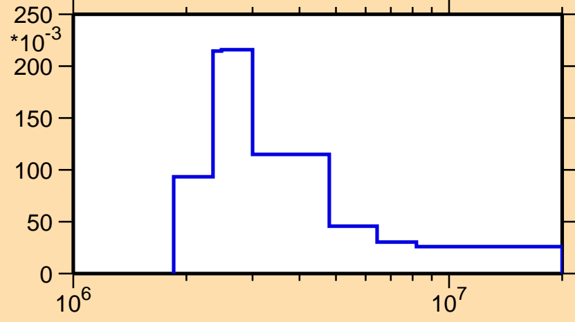
\sigma vs. E for ^{98}\text{Pd}(n,n_3)
