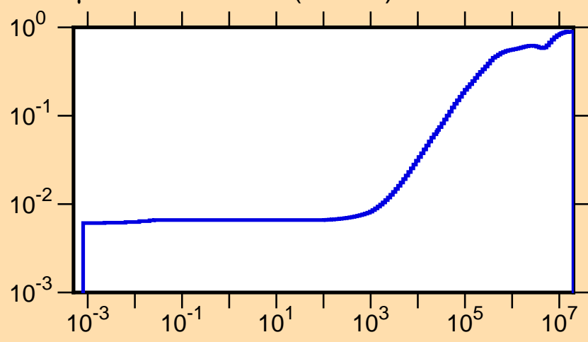
\mu vs. E for ^{111}\text{Pd}(\text{mt251})
