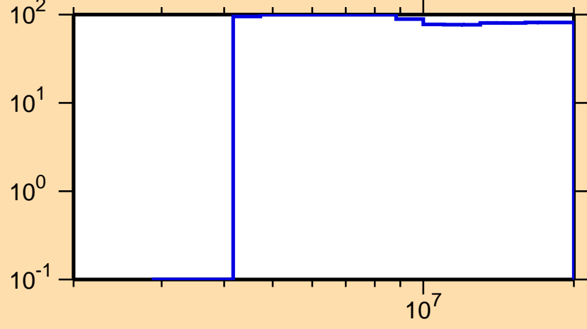
\Delta\sigma/\sigma vs. E for ^{111}\text{Pd}(n,p)
