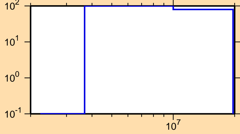
\Delta\sigma/\sigma vs. E for ^{111}\text{Pd}(n,p)
