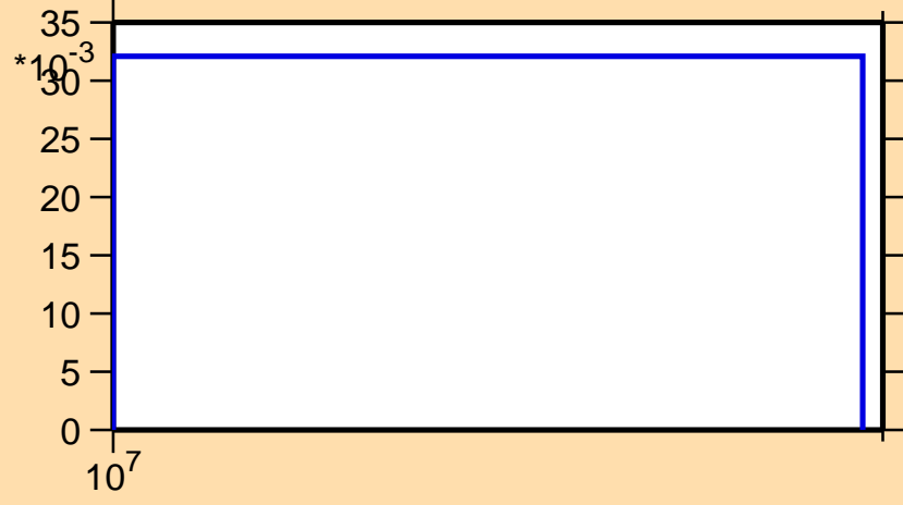
\sigma vs. E for ^{111}\text{Pd}(n,3n)
