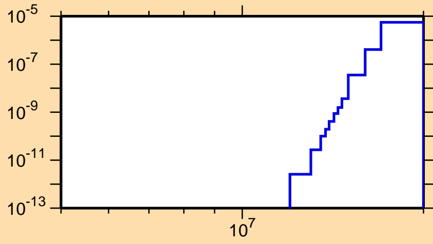
\sigma vs. E for ^{116}\text{Pd}(n,n\alpha)
