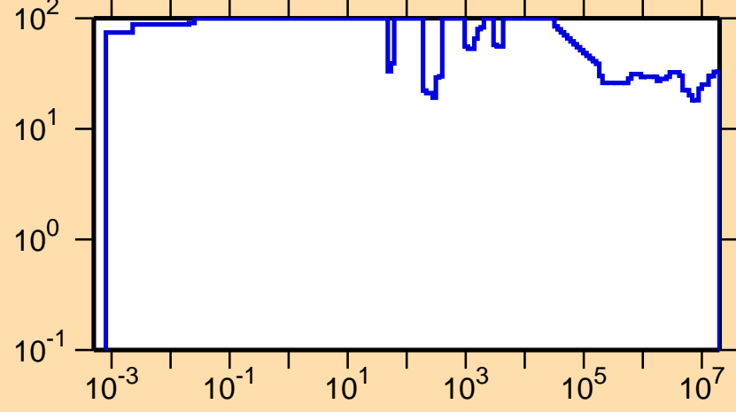
\Delta\sigma/\sigma vs. E for ^{116}\text{Pd}(n,\text{tot.})
