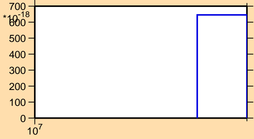
\sigma vs. E for ^{116}\text{Pd}(n,2np)
