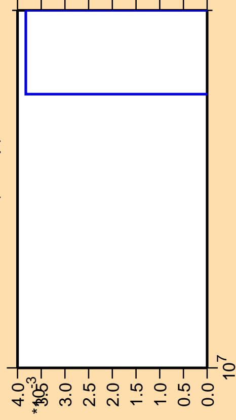
\Delta\sigma/\sigma vs. E for ^{116}\text{Pd}(n,2np)
