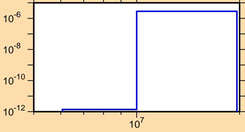
\sigma vs. E for ^{116}\text{Pd}(n,\alpha)
