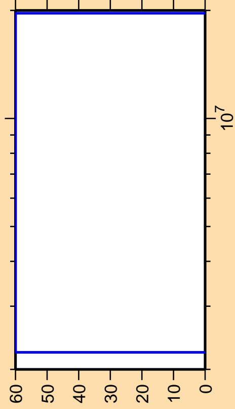
\Delta\sigma/\sigma vs. E for ^{116}\text{Pd}(n,\gamma)
