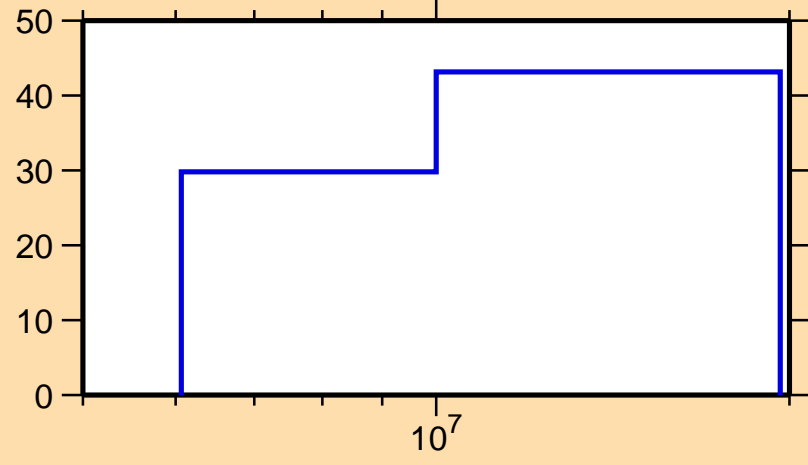
\Delta\sigma/\sigma vs. E for ^{116}\text{Pd}(n,el.)
