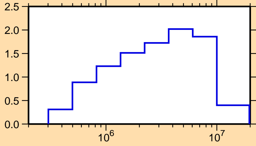
\sigma vs. E for ^{116}\text{Pd}(n,\text{inel.})
