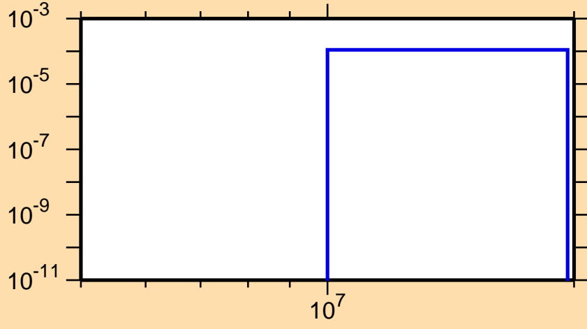
\sigma vs. E for ^{116}\text{Pd}(n,p)
