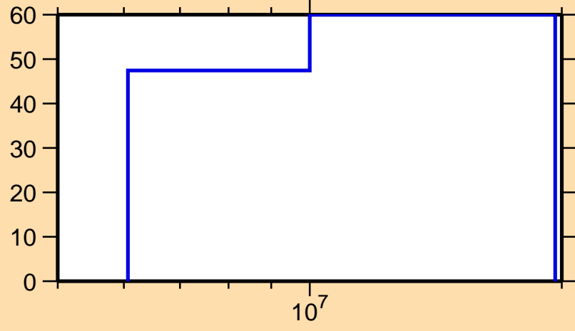
\Delta\sigma/\sigma vs. E for ^{116}\text{Pd}(n,n\text{cont.})
