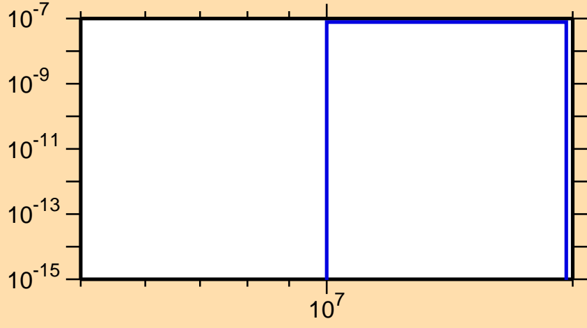
\sigma vs. E for ^{116}\text{Pd}(n,n\alpha)
