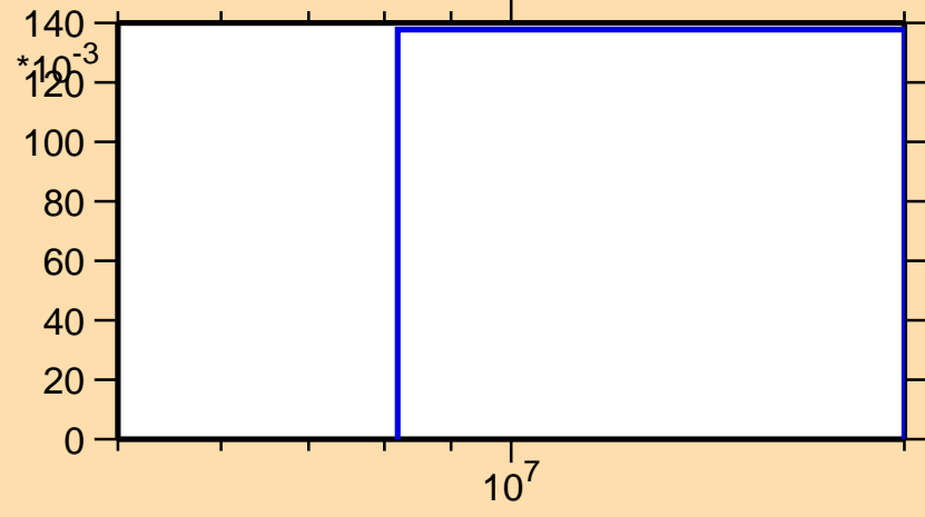
\sigma vs. E for ^{116}\text{Pd}(n,3n)
