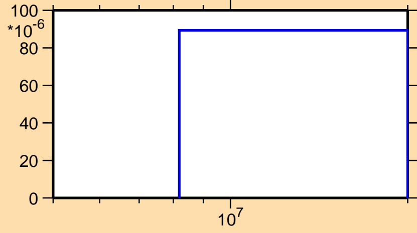
\sigma vs. E for ^{116}\text{Pd}(n,p)
