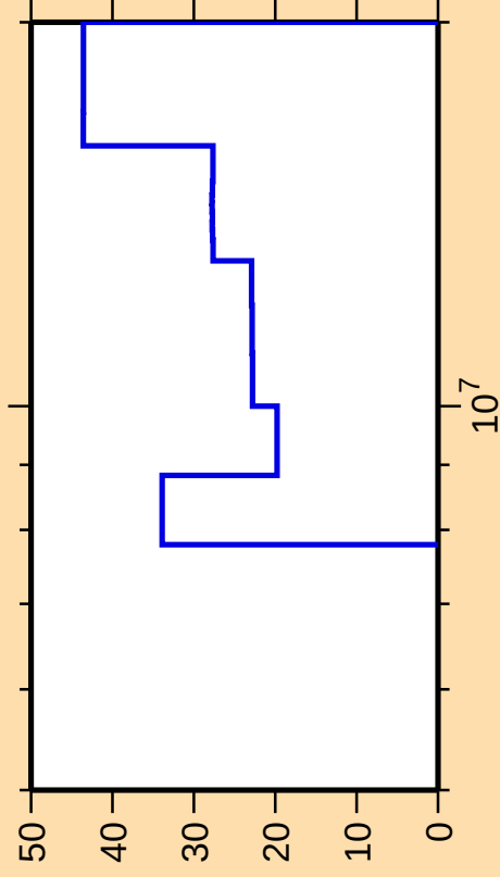
\Delta\sigma/\sigma vs. E for ^{177}\text{Pt}(n,p)
