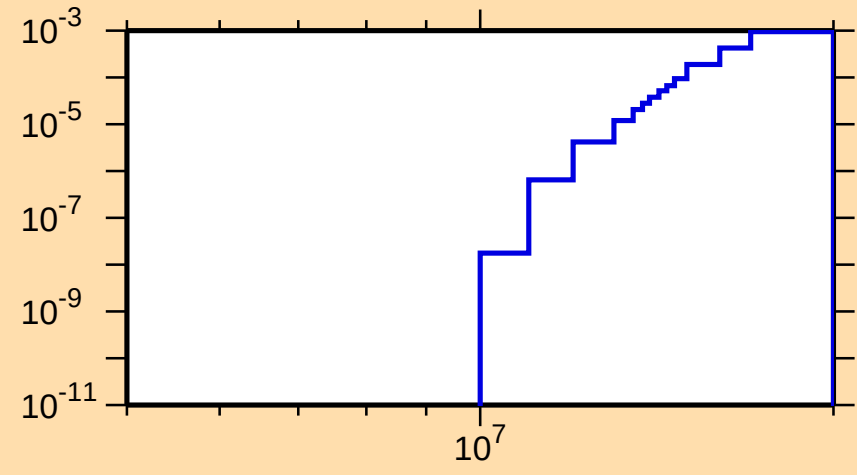
\sigma vs. E for ^{177}\text{Pt}(n,2n\alpha)
