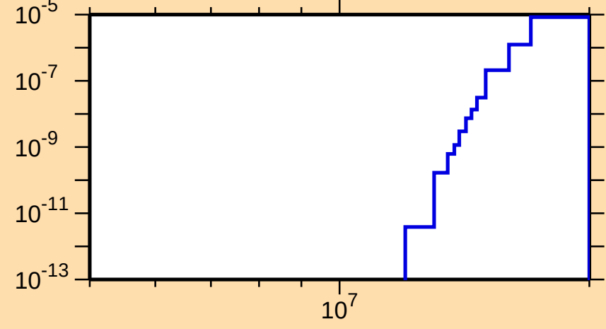
\sigma vs. E for ^{177}\text{Pt}(n,\text{nd})
