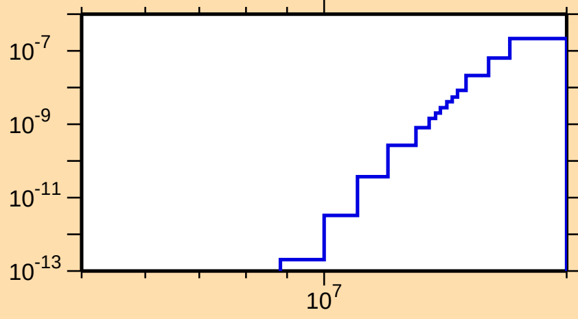
\sigma vs. E for ^{177}\text{Pt}(\text{mt117})
