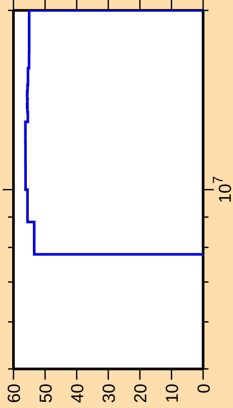
\Delta\sigma/\sigma vs. E for ^{177}\text{Pt}(n,n_1)
