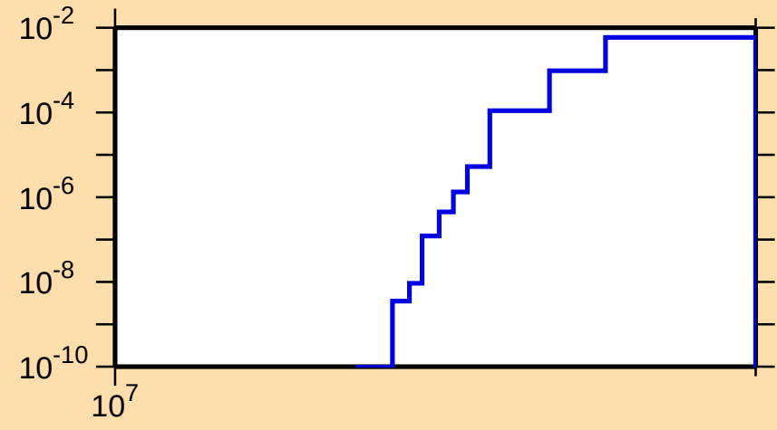
\sigma vs. E for ^{177}\text{Pt}(n,2np)
