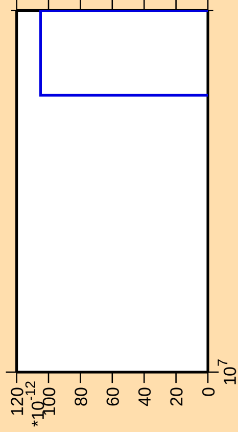
\Delta\sigma/\sigma vs. E for ^{177}\text{Pt}(\text{mt } 11)
