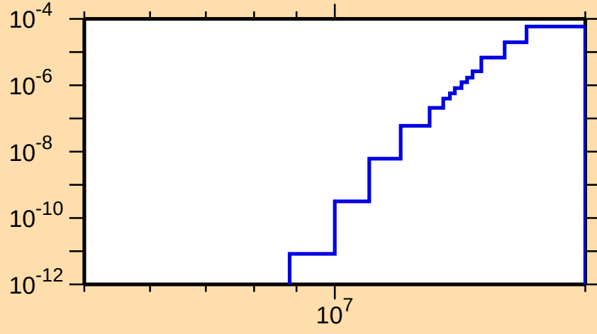
\sigma vs. E for ^{177}\text{Pt}(n,\text{pd})
