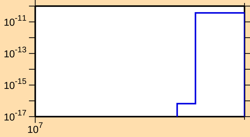
\sigma vs. E for ^{177}\text{Pt}(n,nt)
