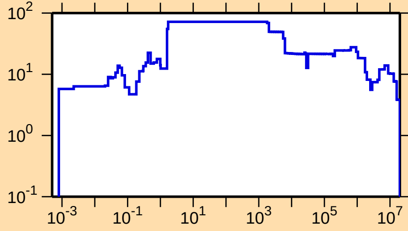
\Delta\sigma/\sigma vs. E for ^{177}\text{Pt}(n,\text{tot.})
