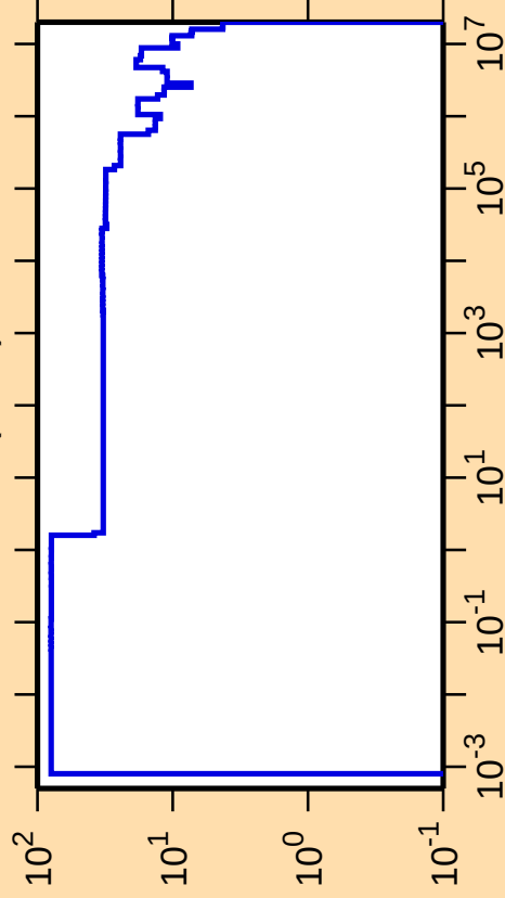
\Delta\sigma/\sigma vs. E for ^{177}\text{Pt}(n,\text{el.})
