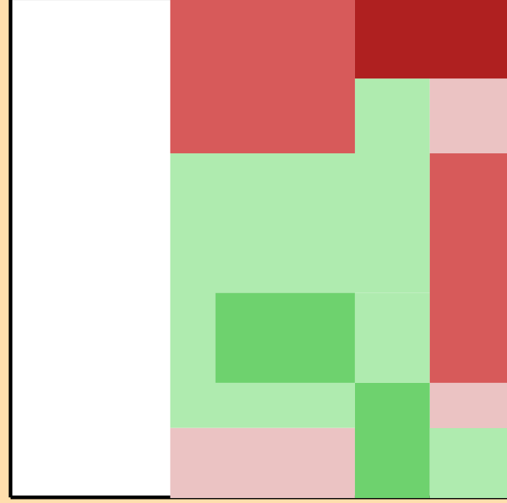
\Delta\sigma/\sigma vs. E for ^{177}\text{Pt}(n,2n)
