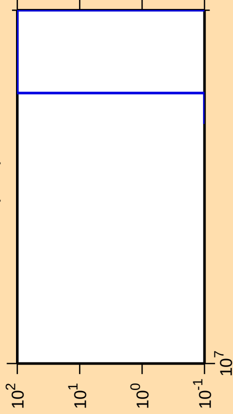
\Delta\sigma/\sigma vs. E for ^{177}\text{Pt}(n,nt)
