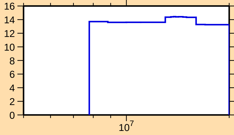
\Delta\sigma/\sigma vs. E for ^{177}\text{Pt}(n,\text{nonel.})
