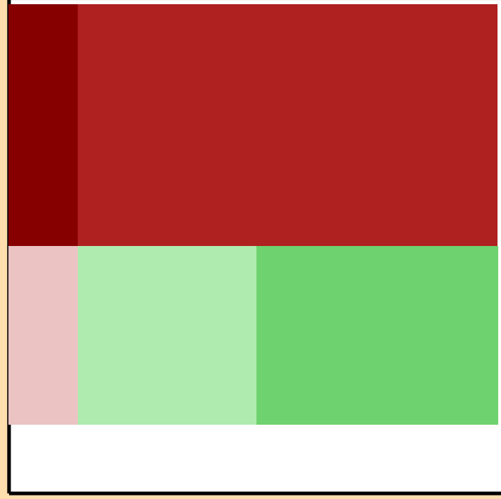
\Delta\sigma/\sigma vs. E for ^{177}\text{Pt}(n,\text{nonel.})
