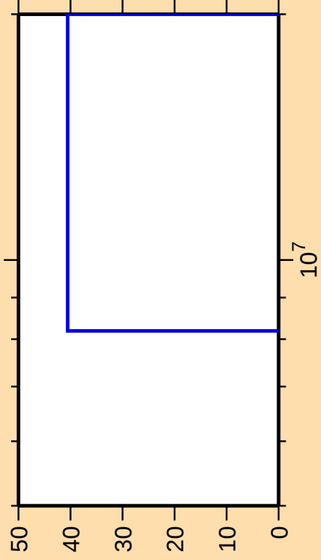
\Delta\sigma/\sigma vs. E for ^{177}\text{Pt}(n,n\text{cont.})
