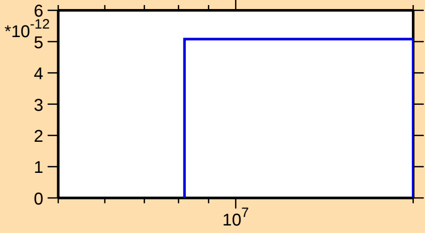
\sigma vs. E for ^{177}\text{Pt}(n,3n)
