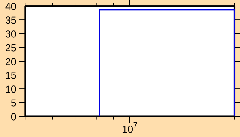
\Delta\sigma/\sigma vs. E for ^{177}\text{Pt}(n,\text{inel.})
