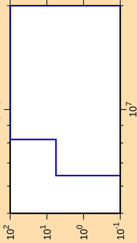
\Delta\sigma/\sigma vs. E for ^{177}\text{Pt}(n,t)
