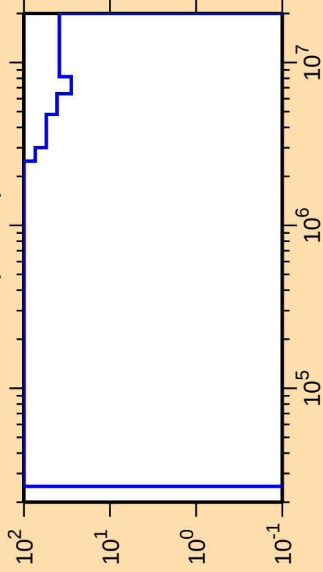
\Delta\sigma/\sigma vs. E for ^{177}\text{Pt}(n,\text{inel.})
