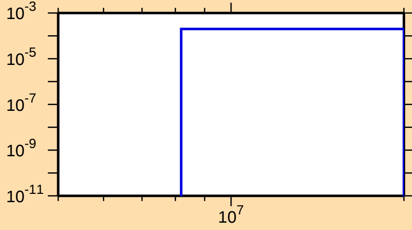
\sigma vs. E for ^{177}\text{Pt}(n,t)
