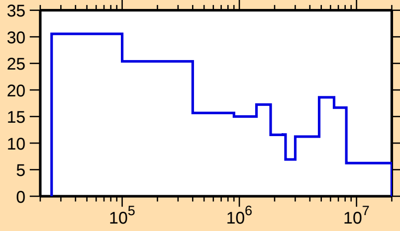
\Delta\sigma/\sigma vs. E for ^{177}\text{Pt}(n,\text{el.})
