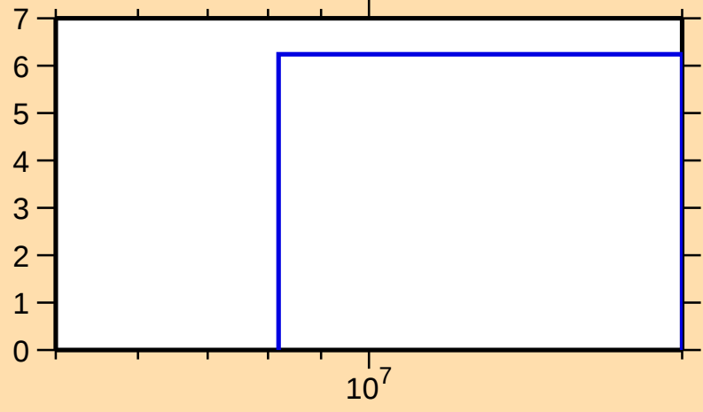
\Delta\sigma/\sigma vs. E for ^{177}\text{Pt}(n,\text{el.})
