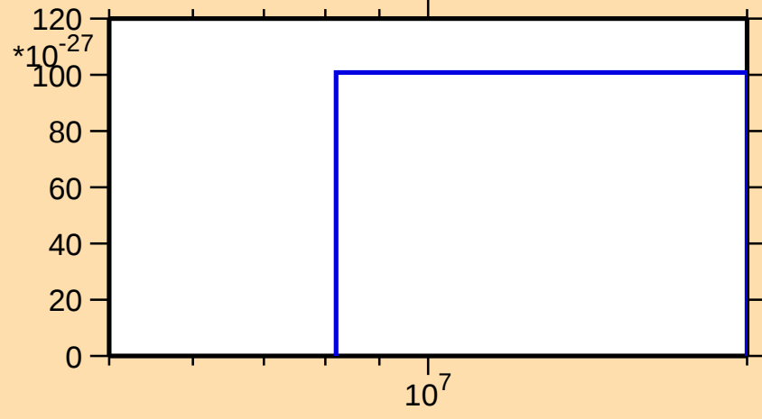
\sigma vs. E for ^{177}\text{Pt}(\text{mt } 11)
