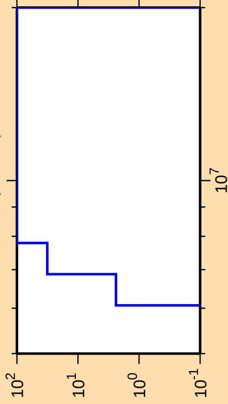
\Delta\sigma/\sigma vs. E for ^{179}\text{Pt}(n,\text{He}3)
