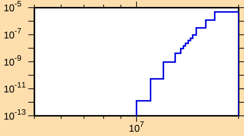
\sigma vs. E for ^{179}\text{Pt}(n,\text{pd})
