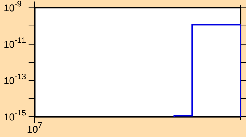
\sigma vs. E for ^{179}\text{Pt}(n,nt)
