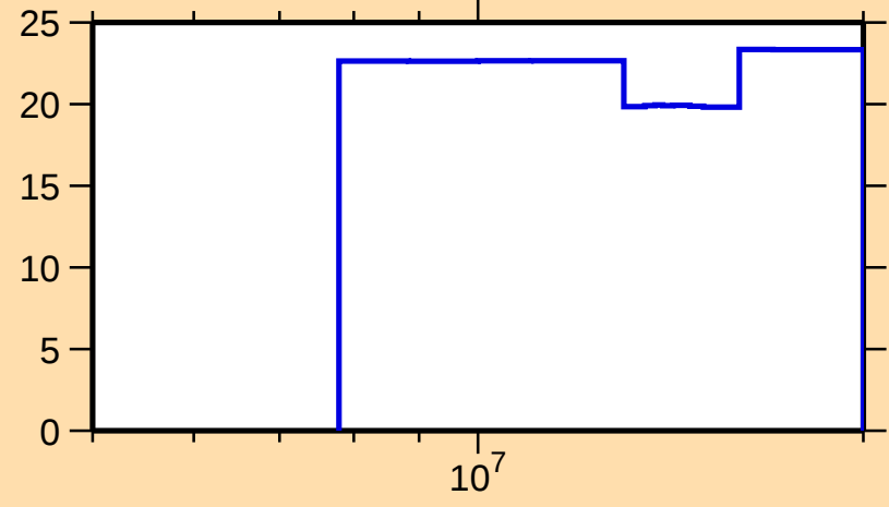
\Delta\sigma/\sigma vs. E for ^{179}\text{Pt}(n,\text{nonel.})
