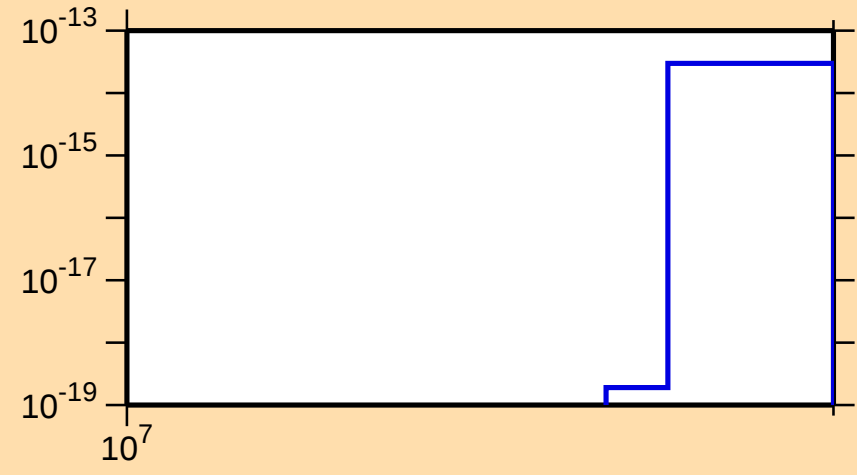
\sigma vs. E for ^{179}\text{Pt}(n,3n\alpha)
