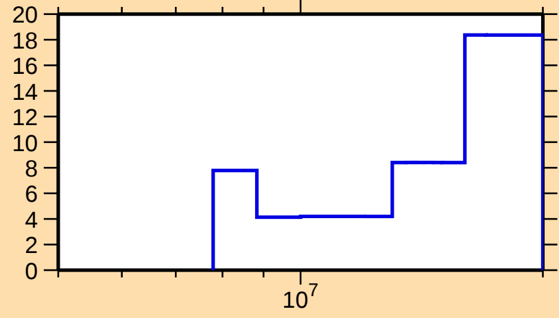
\Delta\sigma/\sigma vs. E for ^{179}\text{Pt}(n,\text{tot.})
