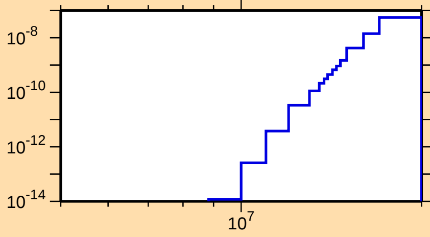
\sigma vs. E for ^{179}\text{Pt}(\text{mt117})
