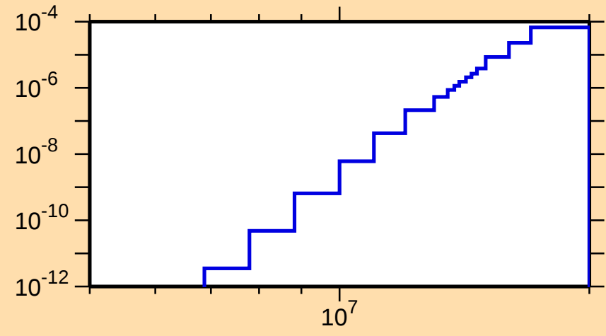
\sigma vs. E for ^{179}\text{Pt}(n,\text{He}3)
