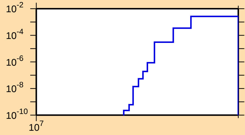
\sigma vs. E for ^{179}\text{Pt}(n,2np)
