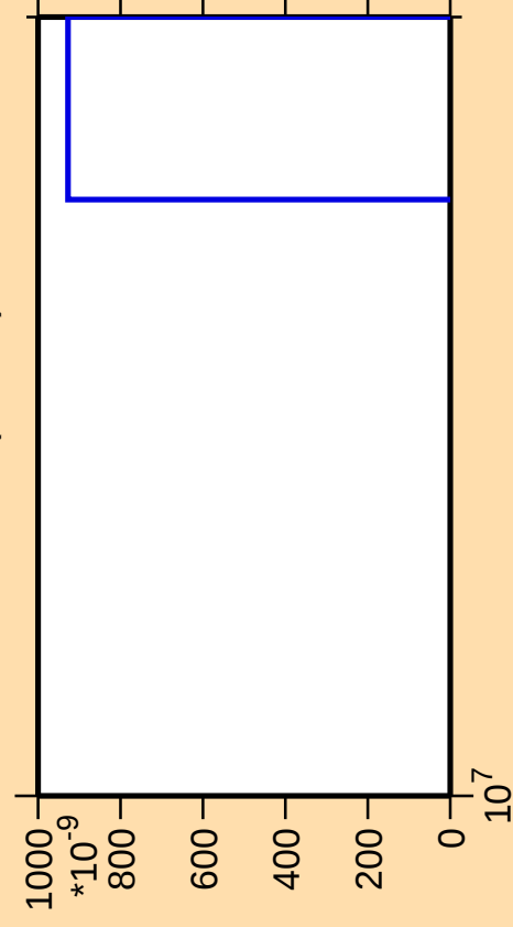
\Delta\sigma/\sigma vs. E for ^{179}\text{Pt}(\text{mt 11})
