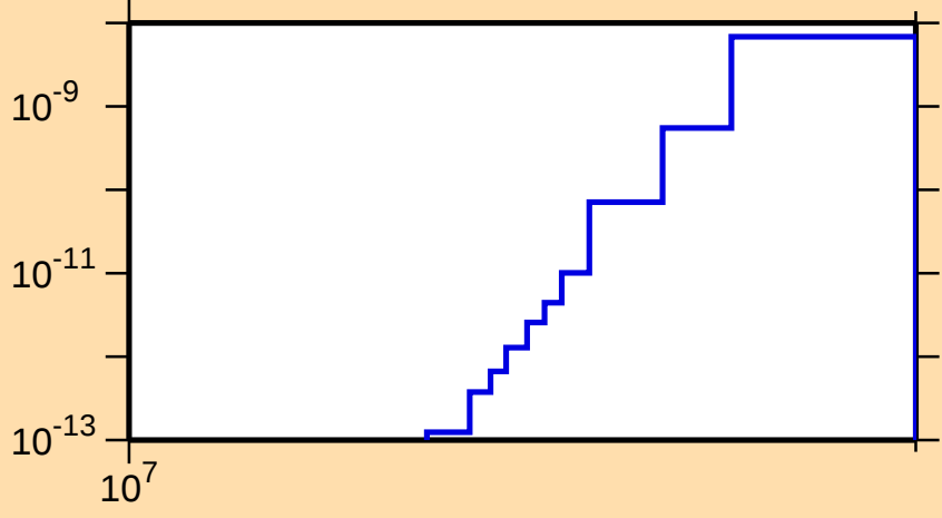
\sigma vs. E for ^{179}\text{Pt}(\text{mt } 34)
