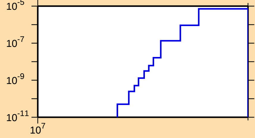
\sigma vs. E for ^{179}\text{Pt}(n,\text{nd})
