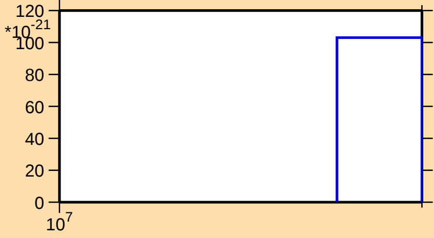
\sigma vs. E for ^{179}\text{Pt}(\text{mt 11})
