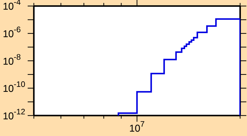
\sigma vs. E for ^{179}\text{Pt}(\text{mt } 45)
