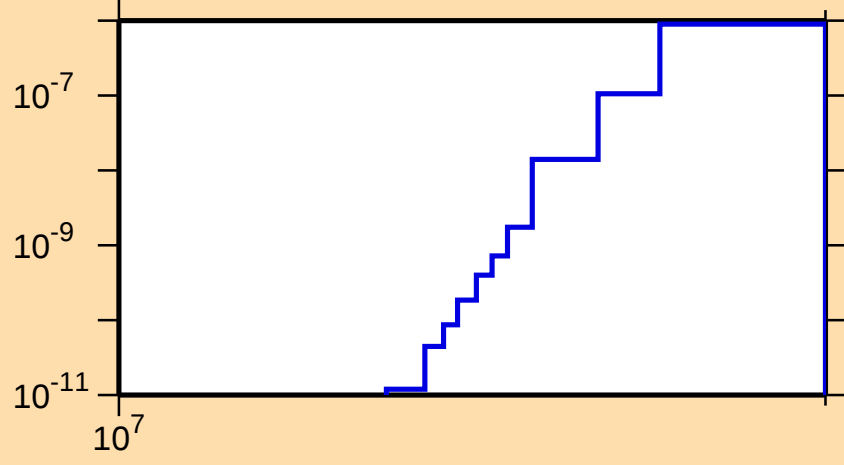
\sigma vs. E for ^{179}\text{Pt}(n,\text{pt})
