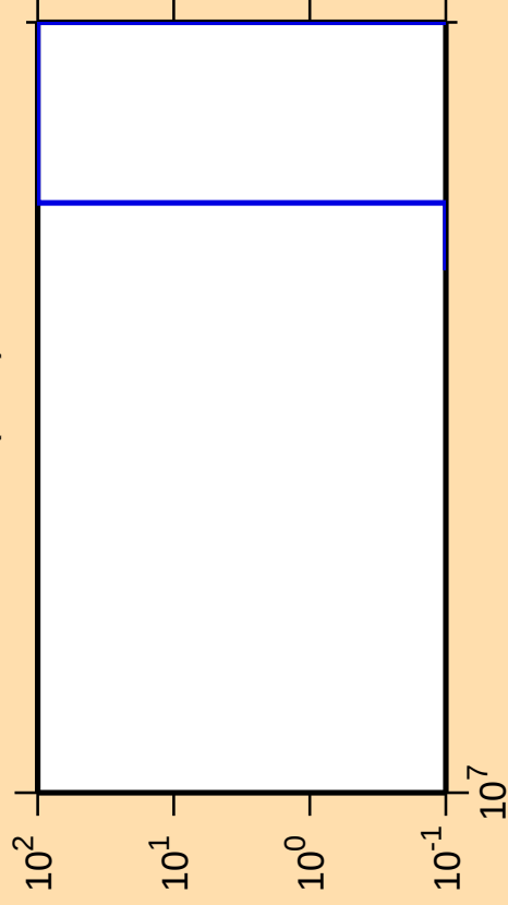
\Delta\sigma/\sigma vs. E for ^{179}\text{Pt}(n,nt)
