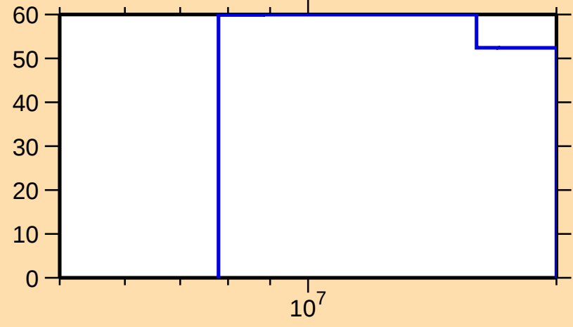
\Delta\sigma/\sigma vs. E for ^{179}\text{Pt}(n,\text{inel.})
