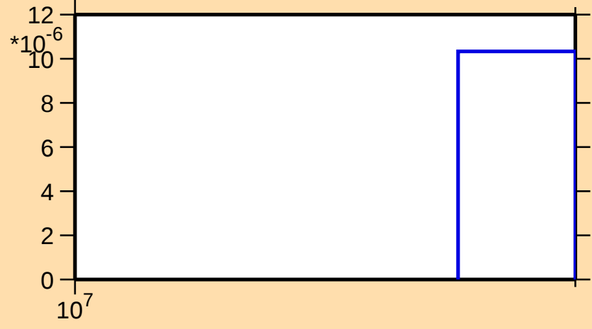
\sigma vs. E for ^{179}\text{Pt}(n,3n)
