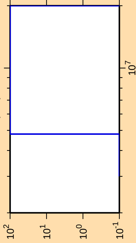
\Delta\sigma/\sigma vs. E for ^{183}\text{Pt}(n,d)
