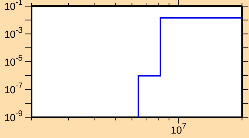
\sigma vs. E for ^{183}\text{Pt}(n,np)
