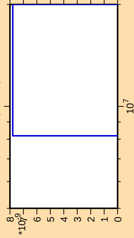
\Delta\sigma/\sigma vs. E for ^{183}\text{Pt}(\text{mt } 11)
