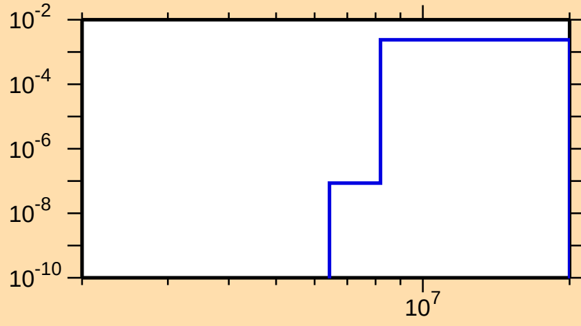
\sigma vs. E for ^{183}\text{Pt}(n,d)
