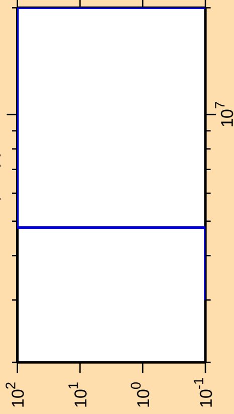
\Delta\sigma/\sigma vs. E for ^{183}\text{Pt}(n,np)
