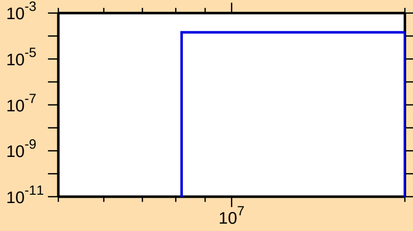
\sigma vs. E for ^{183}\text{Pt}(n,t)
