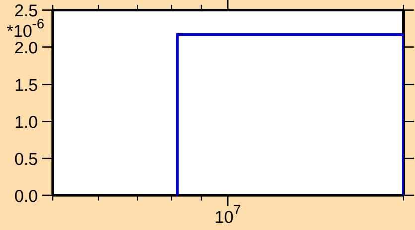
\sigma vs. E for ^{183}\text{Pt}(n,2np)
