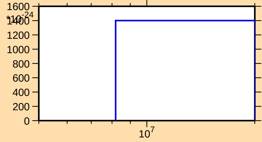
\sigma vs. E for ^{183}\text{Pt}(\text{mt } 11)
