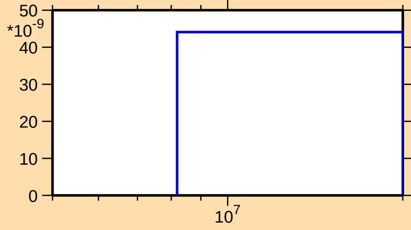
\sigma vs. E for ^{183}\text{Pt}(n,\text{nd})
