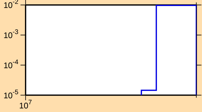
\sigma vs. E for ^{186}\text{Pt}(n,3n)
