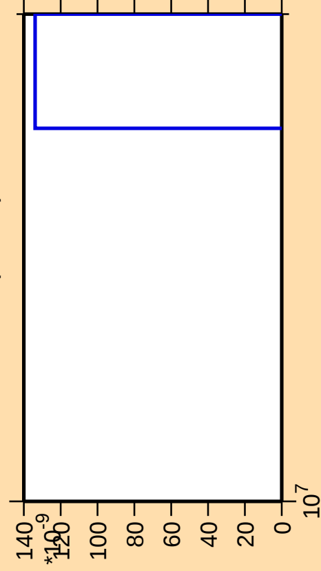
\Delta\sigma/\sigma vs. E for ^{186}\text{Pt}(\text{mt } 11)
