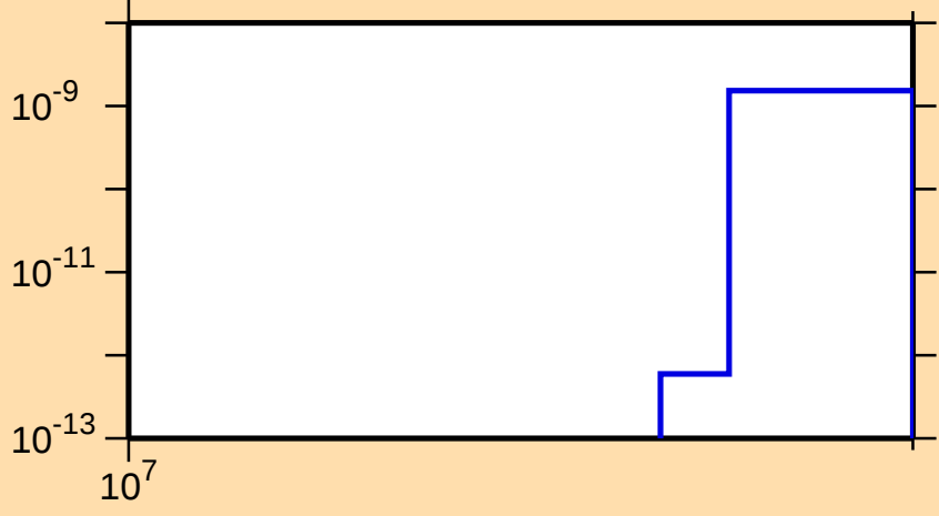
\sigma vs. E for ^{186}\text{Pt}(n,nt)
