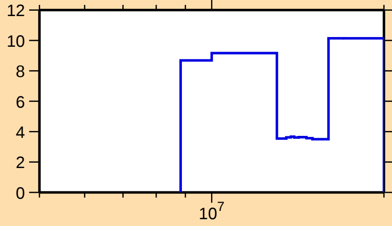
\Delta\sigma/\sigma vs. E for ^{186}\text{Pt}(n,\text{tot.})
