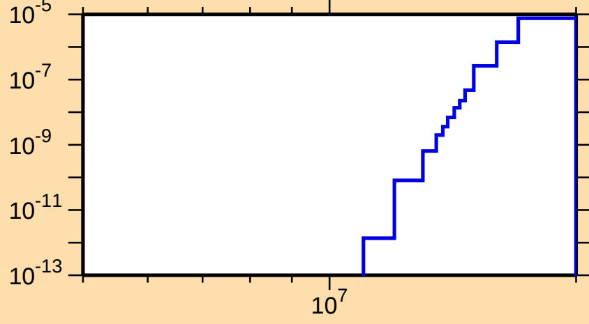
\sigma vs. E for ^{186}\text{Pt}(n,2n\alpha)
