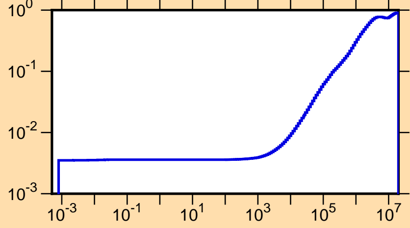
\mu vs. E for ^{192}\text{Pt}(\text{mt251})
