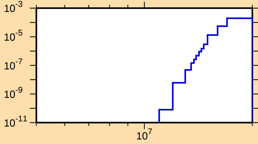
\sigma vs. E for ^{192}\text{Pt}(n,t)
