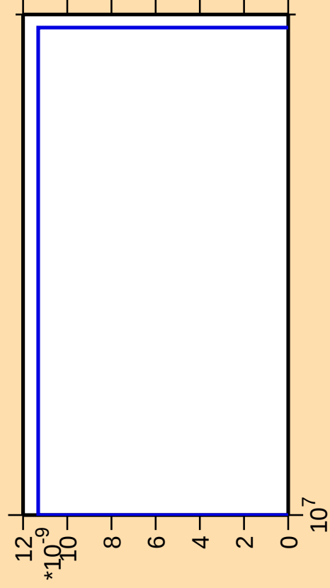
\Delta\sigma/\sigma vs. E for ^{192}\text{Pt}(\text{mt } 11)
