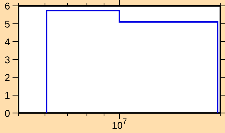
\Delta\sigma/\sigma vs. E for ^{192}\text{Pt}(n,\text{nonel.})
