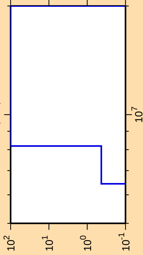
\Delta\sigma/\sigma vs. E for ^{192}\text{Pt}(n,d)
