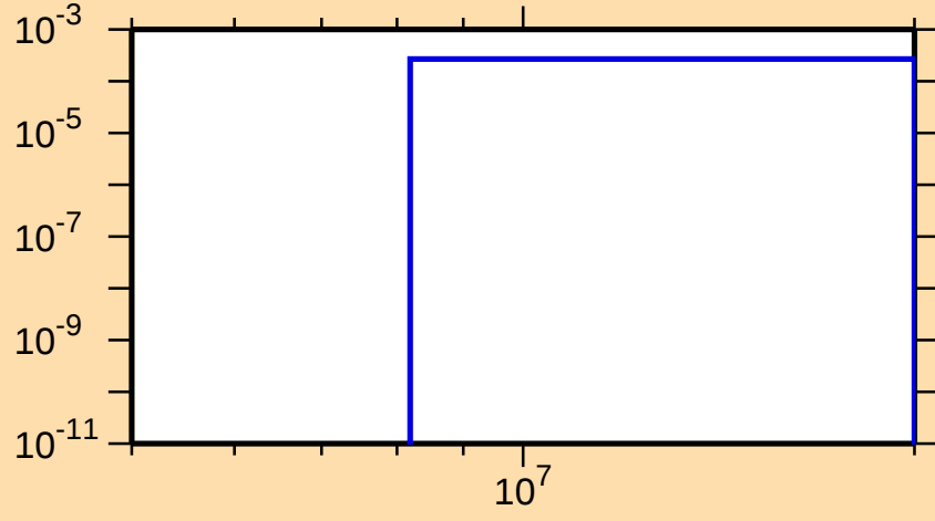
\sigma vs. E for ^{192}\text{Pt}(n,d)
