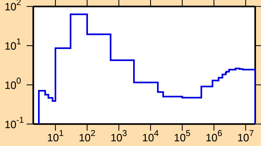
\sigma vs. E for ^{192}\text{Pt}(n,\text{nonel.})
