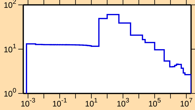
\sigma vs. E for ^{192}\text{Pt}(n,\text{el.})
