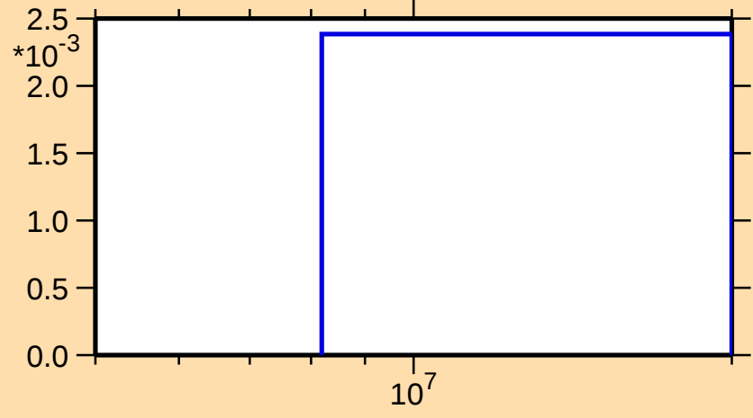
\sigma vs. E for ^{192}\text{Pt}(n,3n)
