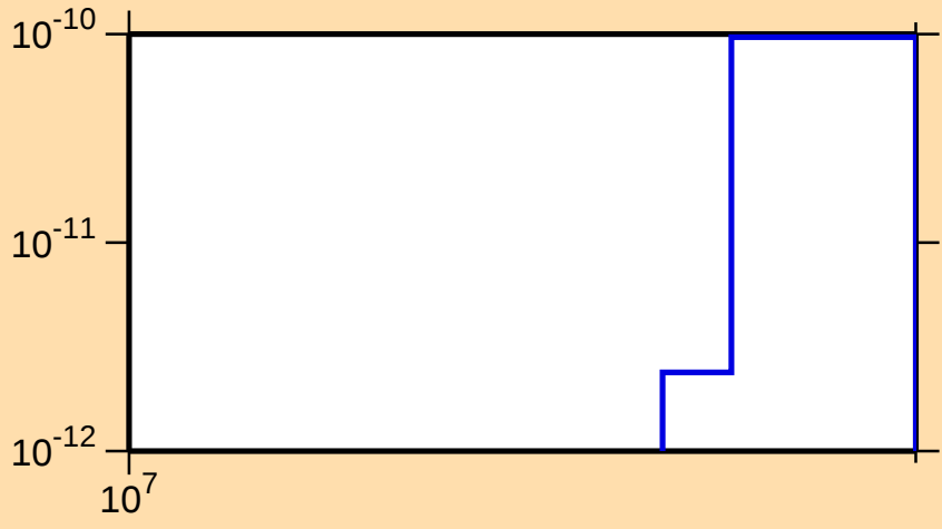
\sigma vs. E for ^{195}\text{Pt}(n,\text{He3})
