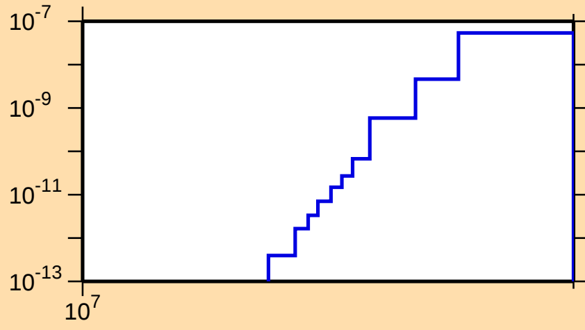
\sigma vs. E for ^{195}\text{Pt}(n,2n\alpha)
