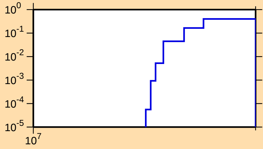
\sigma vs. E for ^{195}\text{Pt}(n,3n)
