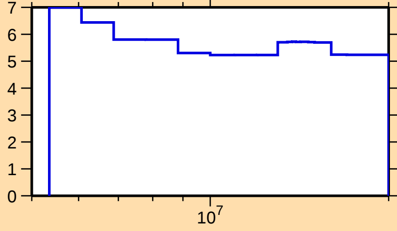
\Delta\sigma/\sigma vs. E for ^{195}\text{Pt}(n,\text{nonel.})
