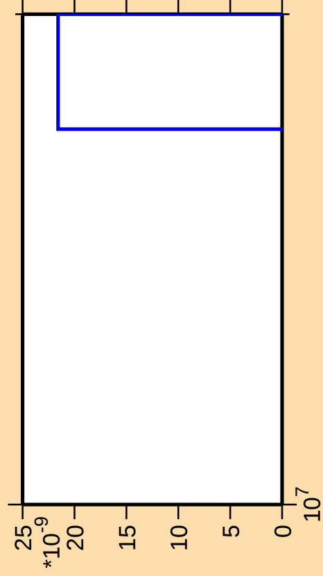
\Delta\sigma/\sigma vs. E for ^{195}\text{Pt}(\text{mt } 11)
