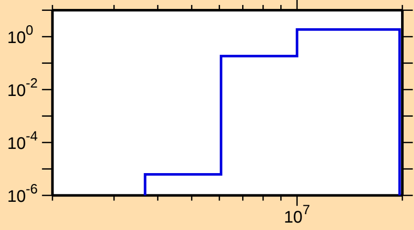
\sigma vs. E for ^{195}\text{Pt}(n,2n)
