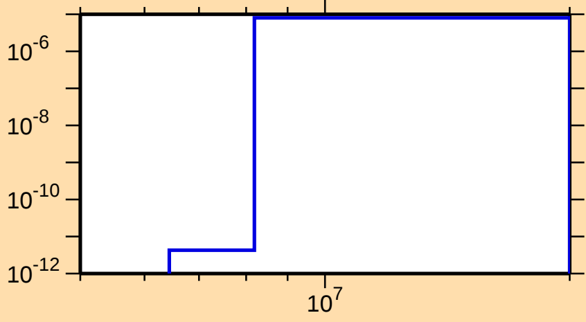
\sigma vs. E for ^{195}\text{Pt}(n,n\alpha)
