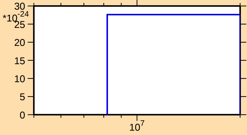
\sigma vs. E for ^{195}\text{Pt}(\text{mt 11})
