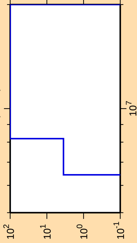
\Delta\sigma/\sigma vs. E for ^{195}\text{Pt}(n,n\alpha)
