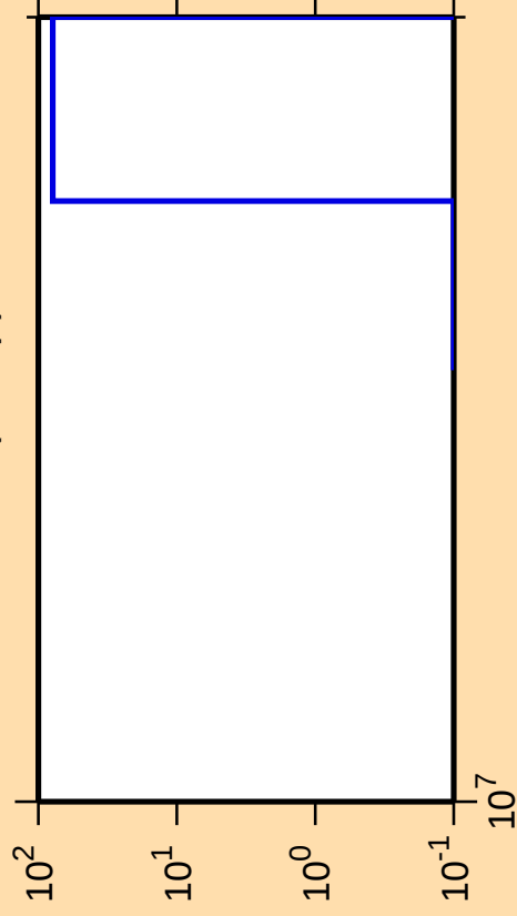
\Delta\sigma/\sigma vs. E for ^{201}\text{Pt}(n,2np)
