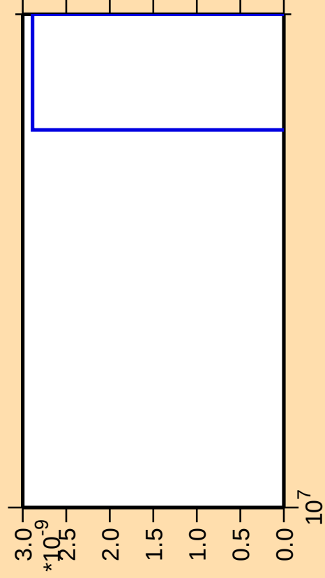
\Delta\sigma/\sigma vs. E for ^{201}\text{Pt}(\text{mt } 11)
