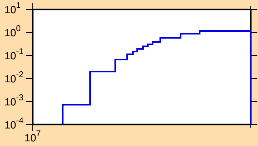
\sigma vs. E for ^{204}\text{Pt}(n,3n)
