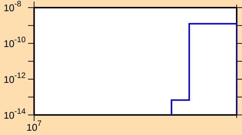
\sigma vs. E for ^{204}\text{Pt}(n,nt)
