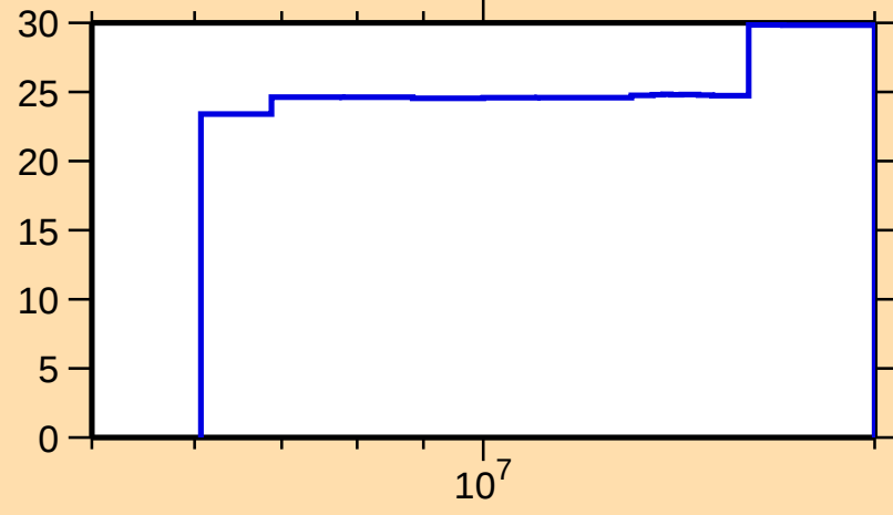
\Delta\sigma/\sigma vs. E for ^{204}\text{Pt}(n,\text{nonel.})
