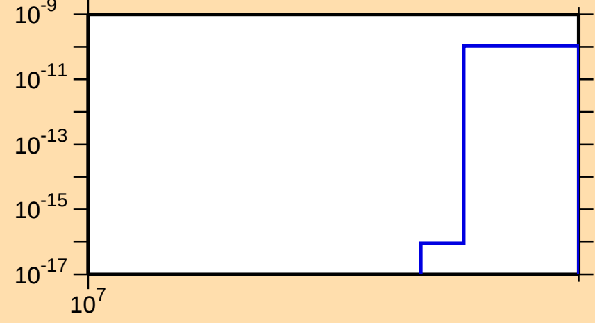
\sigma vs. E for ^{204}\text{Pt}(n,\text{nd})
