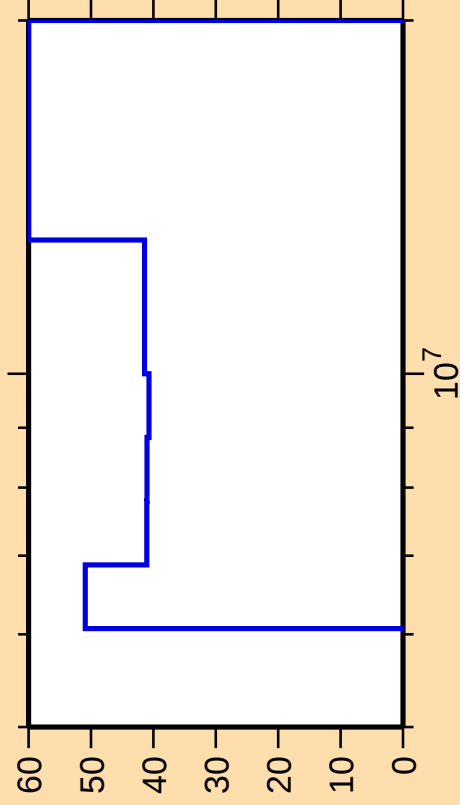
\Delta\sigma/\sigma vs. E for ^{204}\text{Pt}(n,2n)
