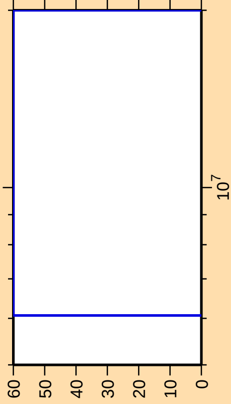
\Delta\sigma/\sigma vs. E for ^{204}\text{Pt}(n,\gamma)
