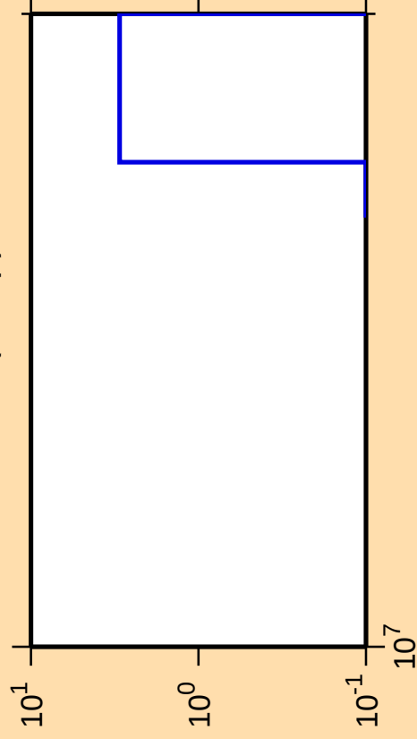
\Delta\sigma/\sigma vs. E for ^{204}\text{Pt}(n,2np)
