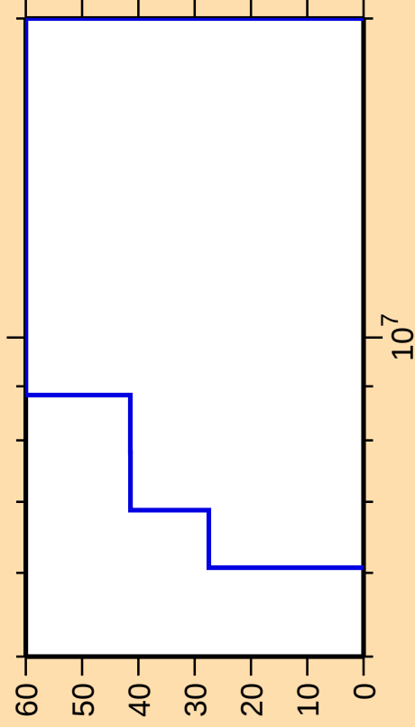
\Delta\sigma/\sigma vs. E for ^{204}\text{Pt}(n,n\text{cont.})
