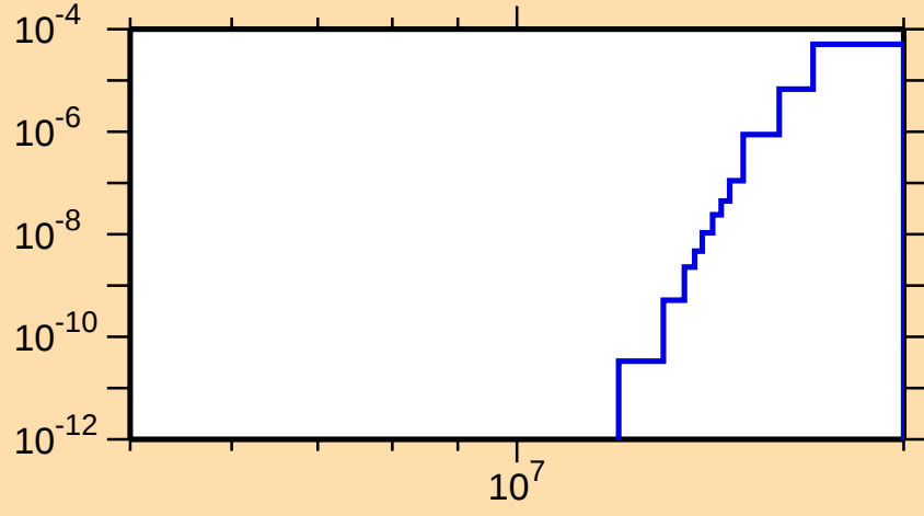
\sigma vs. E for ^{204}\text{Pt}(n,d)
