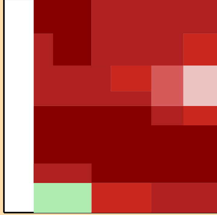
\Delta\sigma/\sigma vs. E for ^{204}\text{Pt}(n,2n)
