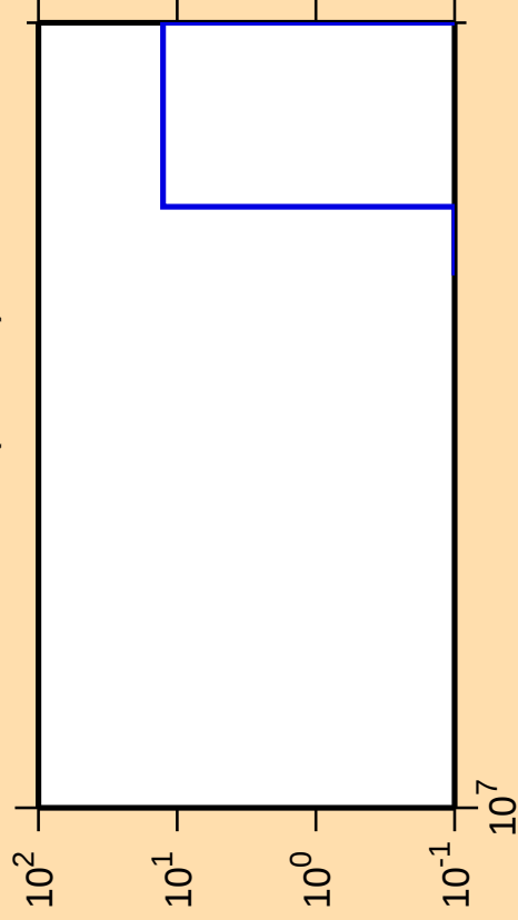
\Delta\sigma/\sigma vs. E for ^{204}\text{Pt}(n,2n\alpha)
