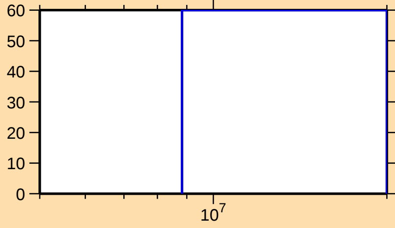
\Delta\sigma/\sigma vs. E for ^{204}\text{Pt}(n,n\text{cont.})
