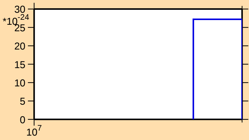
\sigma vs. E for ^{204}\text{Pt}(\text{mt } 11)
