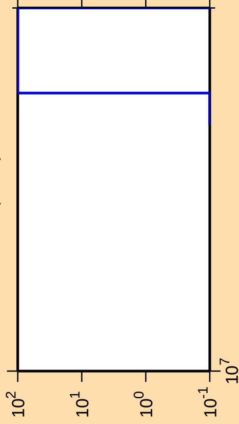
\Delta\sigma/\sigma vs. E for ^{204}\text{Pt}(n,\text{nd})
