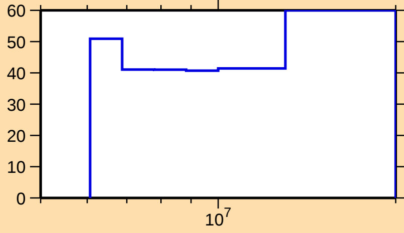
\Delta\sigma/\sigma vs. E for ^{204}\text{Pt}(n,2n)
