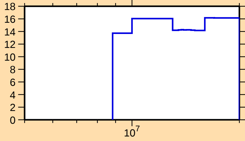
\Delta\sigma/\sigma vs. E for ^{204}\text{Pt}(n,\text{tot.})
