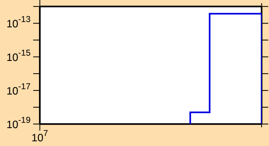
\sigma vs. E for ^{204}\text{Pt}(n,2np)
