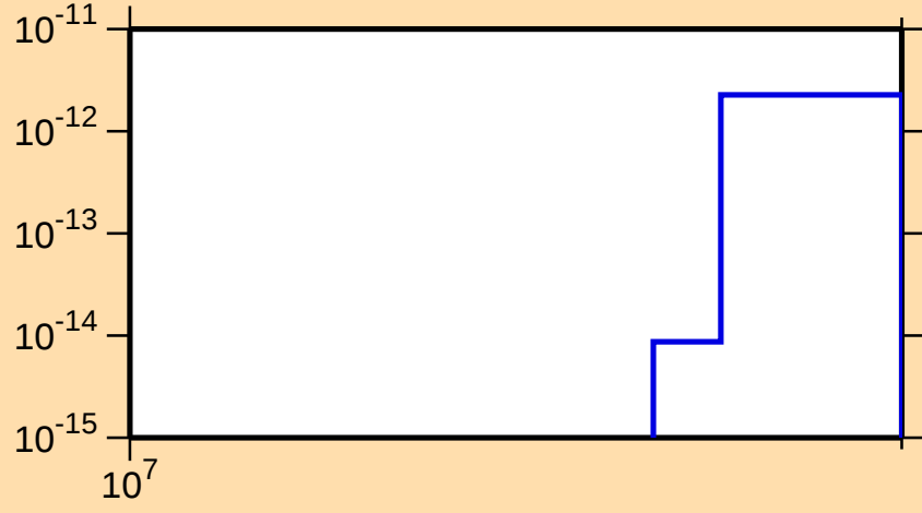
\sigma vs. E for ^{204}\text{Pt}(n,2n\alpha)
