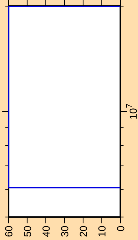
\Delta\sigma/\sigma vs. E for ^{204}\text{Pt}(n,n_1)
