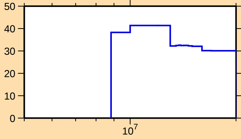
\Delta\sigma/\sigma vs. E for ^{204}\text{Pt}(n,\text{el.})
