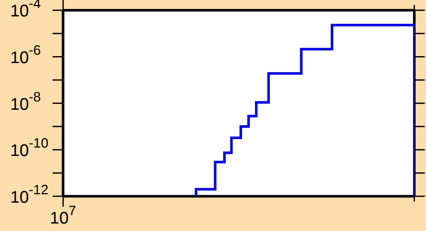
\sigma vs. E for ^{204}\text{Pt}(n,np)
