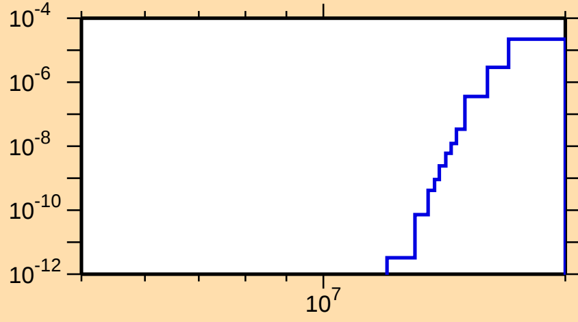
\sigma vs. E for ^{204}\text{Pt}(n,t)
