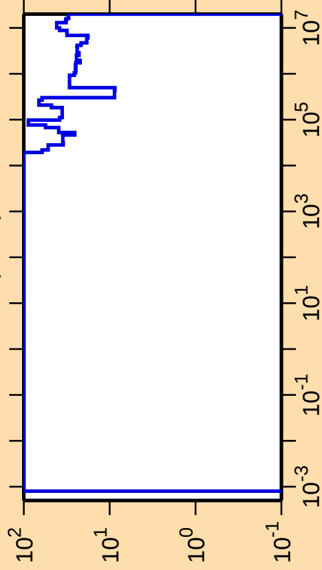
\Delta\sigma/\sigma vs. E for ^{204}\text{Pt}(n,\text{el.})
