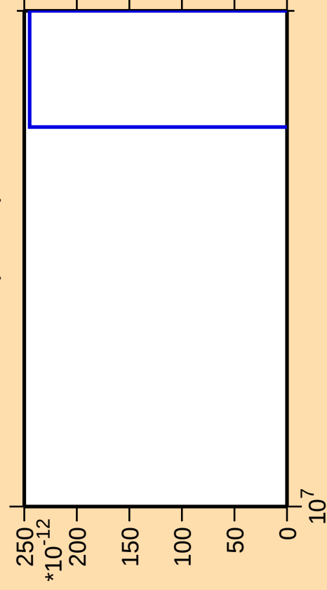
\Delta\sigma/\sigma vs. E for ^{204}\text{Pt}(\text{mt } 11)
