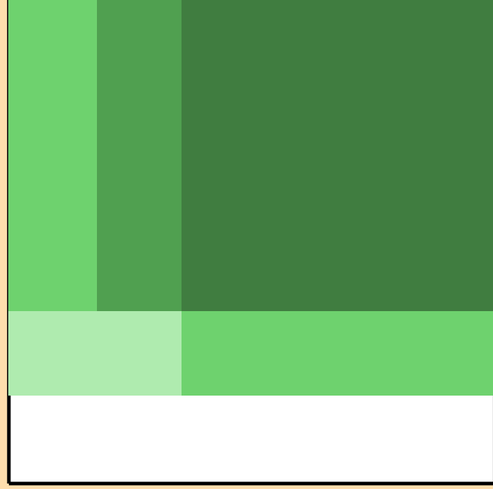
\Delta\sigma/\sigma vs. E for ^{226}\text{Ra}(n,\text{tot.})
