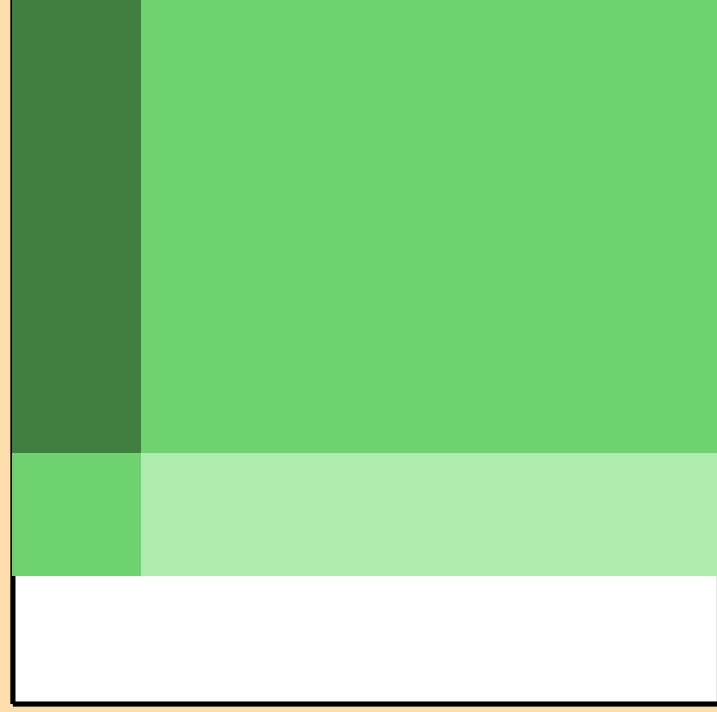
\Delta\sigma/\sigma vs. E for ^{226}\text{Ra}(n,\text{nonel.})
