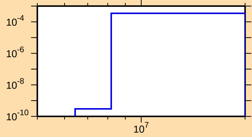
\sigma vs. E for ^{226}\text{Ra}(n,p)
