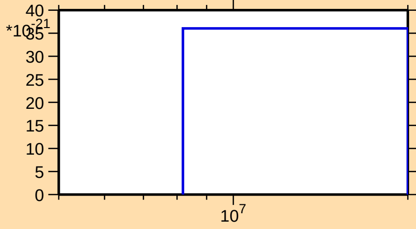
\sigma vs. E for ^{226}\text{Ra}(\text{mt } 42)
