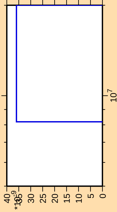
\Delta\sigma/\sigma vs. E for ^{226}\text{Ra}(\text{mt } 42)
