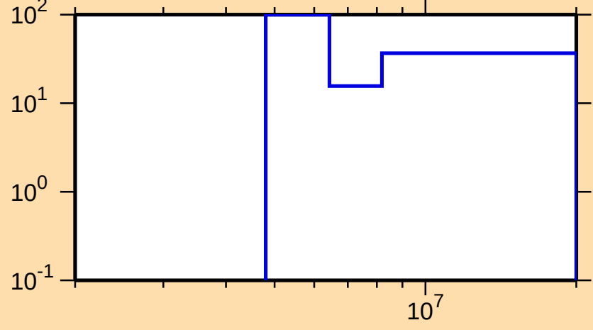
\Delta\sigma/\sigma vs. E for ^{226}\text{Ra}(n,2n)
