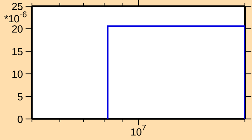
\sigma vs. E for ^{226}\text{Ra}(n,d)
