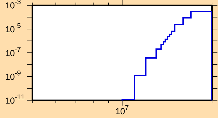
\sigma vs. E for ^{228}\text{Ra}(n,d)
