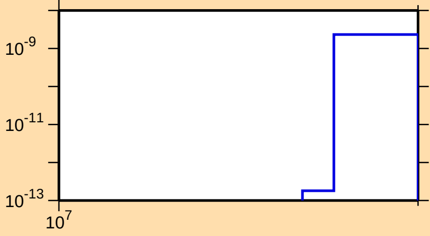
\sigma vs. E for ^{228}\text{Ra}(n,2np)
