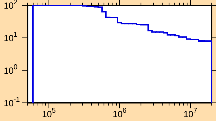
\Delta\sigma/\sigma vs. E for ^{228}\text{Ra}(n,\text{nonel.})
