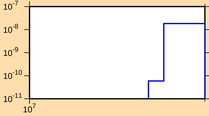
\sigma vs. E for ^{228}\text{Ra}(n,\text{nd})
