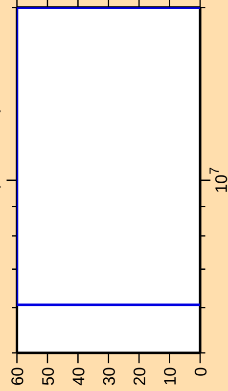
\Delta\sigma/\sigma vs. E for ^{228}\text{Ra}(n,n\text{cont.})
