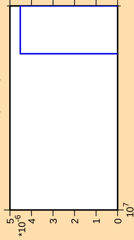
\Delta\sigma/\sigma vs. E for ^{228}\text{Ra}(\text{mt } 42)
