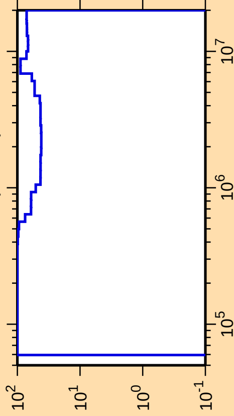
\Delta\sigma/\sigma vs. E for ^{228}\text{Ra}(n,\text{inel.})
