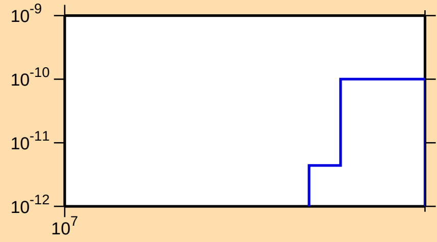
\sigma vs. E for ^{228}\text{Ra}(n,3n\alpha)
