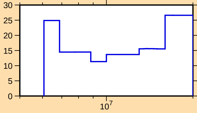
\Delta\sigma/\sigma vs. E for ^{228}\text{Ra}(n,\text{el.})
