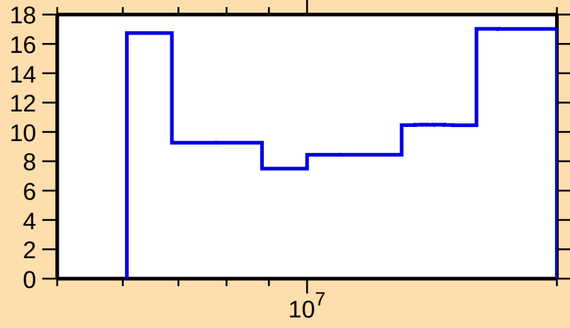
\Delta\sigma/\sigma vs. E for ^{228}\text{Ra}(n,\text{tot.})
