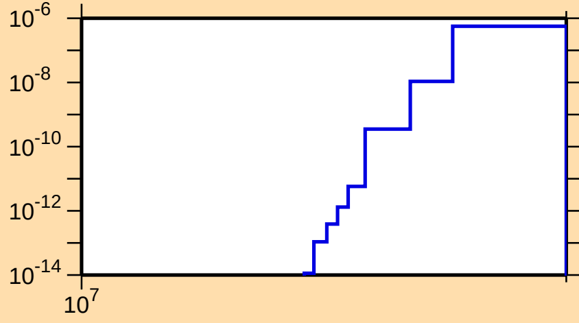
\sigma vs. E for ^{228}\text{Ra}(n,\text{nt})
