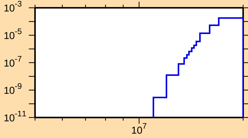
\sigma vs. E for ^{228}\text{Ra}(n,t)
