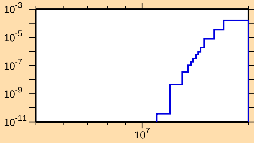
\sigma vs. E for ^{228}\text{Ra}(n,np)
