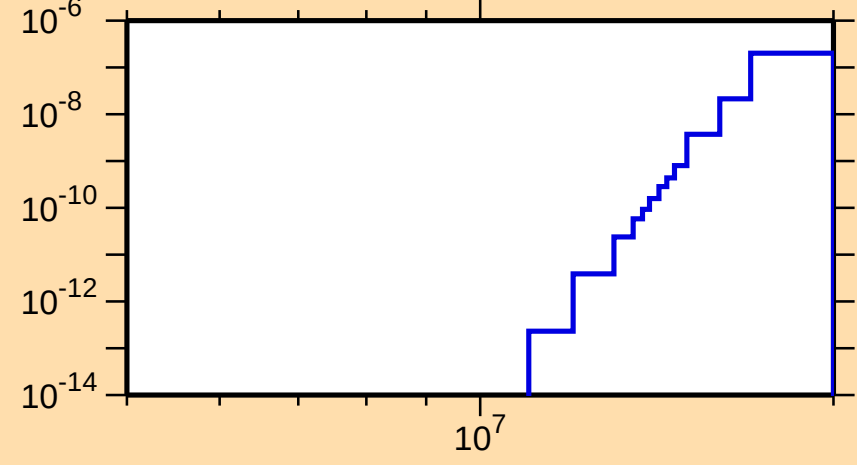
\sigma vs. E for ^{228}\text{Ra}(n,2n\alpha)
