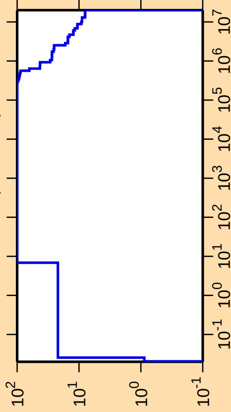
\Delta\sigma/\sigma vs. E for ^{228}\text{Ra}(n,\text{nonel.})
