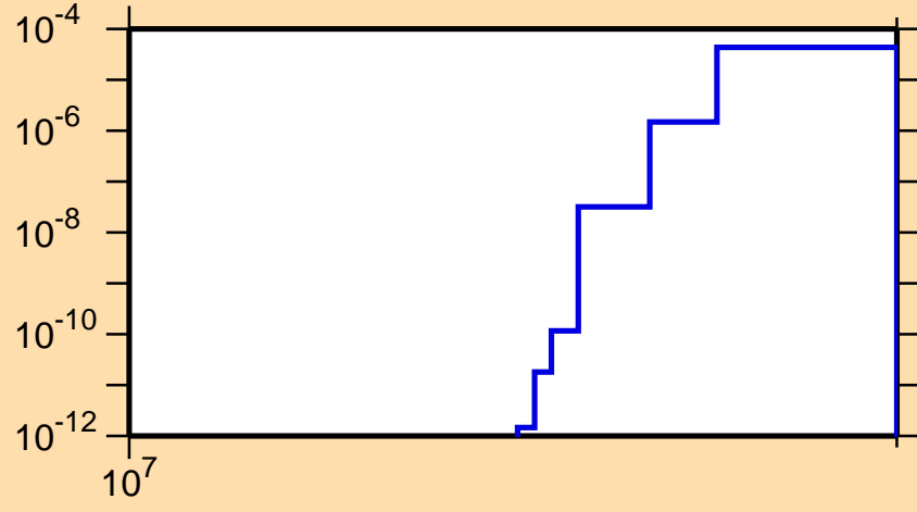
\sigma vs. E for ^{76}\text{Rb}(n,pt)
