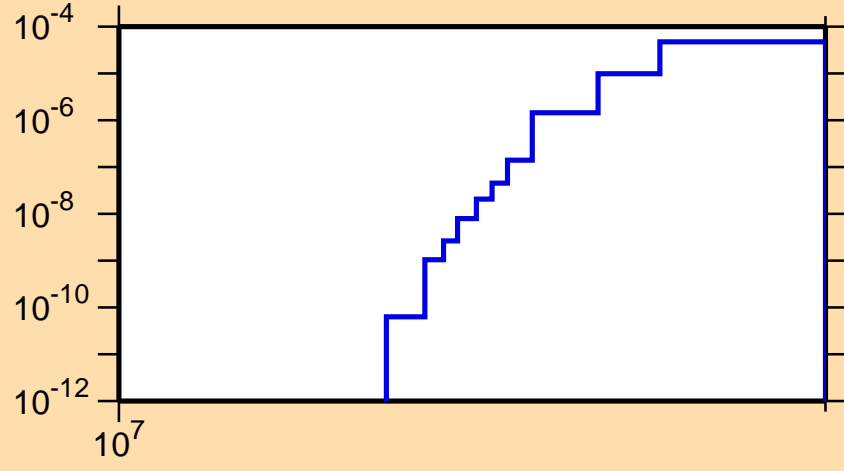
\sigma vs. E for ^{76}\text{Rb}(n,nd)
