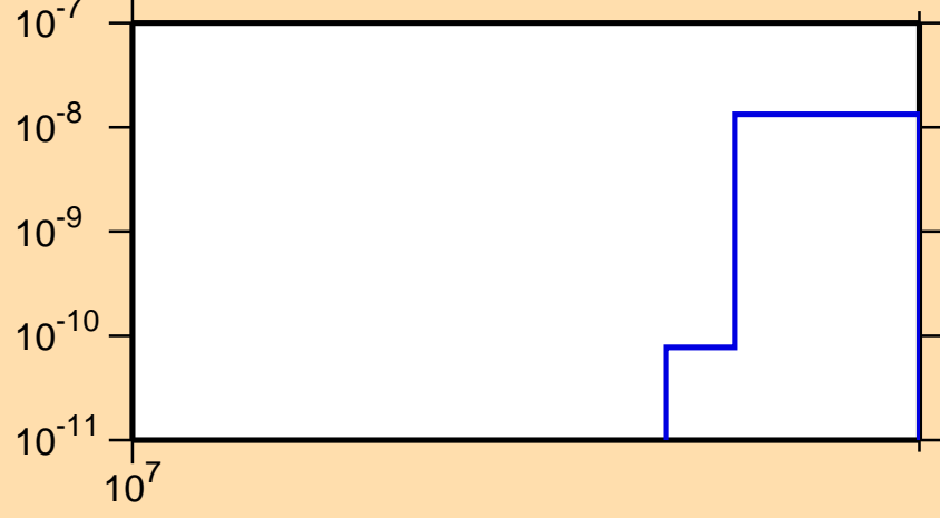
\sigma vs. E for ^{76}\text{Rb} (mt 34)
