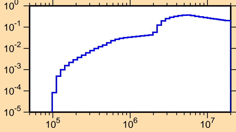
\sigma vs. E for ^{76}\text{Rb}(n,\text{inel.})
