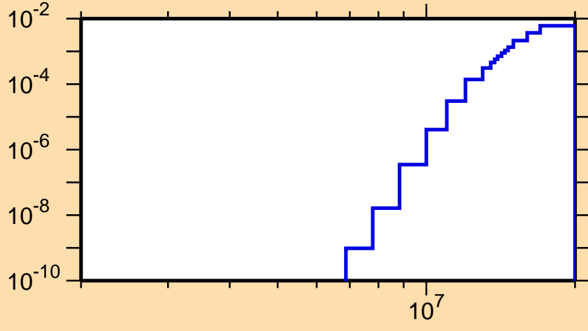
\sigma vs. E for ^{76}\text{Rb}(n,\text{He}3)
