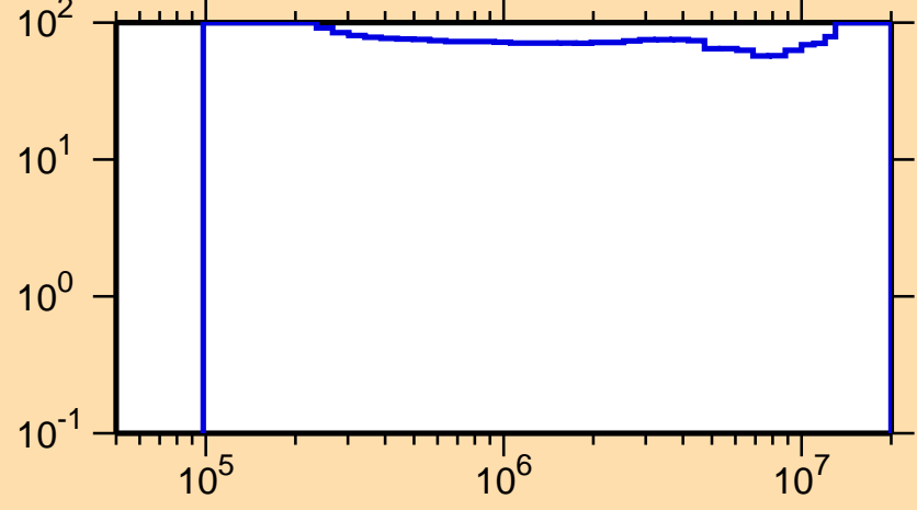
\Delta\sigma/\sigma vs. E for ^{76}\text{Rb}(n,n_1)
