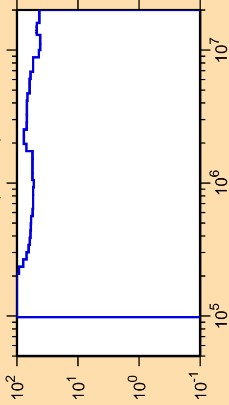
\Delta\sigma/\sigma vs. E for ^{76}\text{Rb}(n,\text{inel.})
