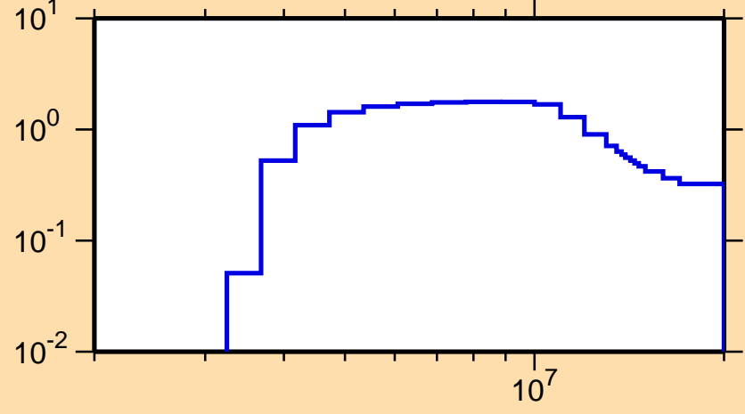
\sigma vs. E for ^{87}\text{Rb}(n,n\text{cont.})
