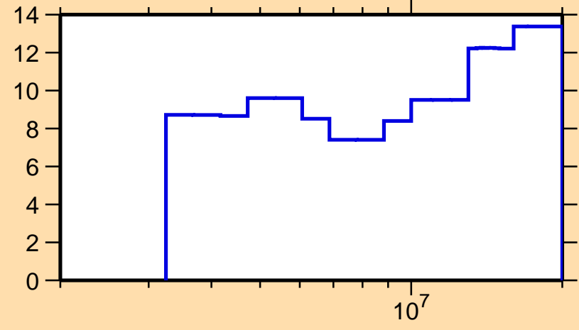
\Delta\sigma/\sigma vs. E for ^{87}\text{Rb}(n,el.)
