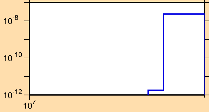
\sigma vs. E for ^{87}\text{Rb}(n,nd)
