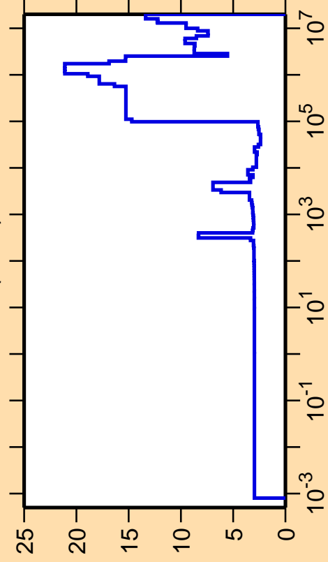
\Delta\sigma/\sigma vs. E for ^{87}\text{Rb}(n,\text{el.})
