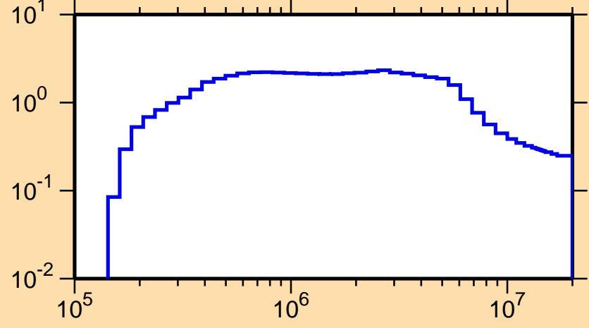
\sigma vs. E for ^{92}\text{Rb}(n,\text{inel.})
