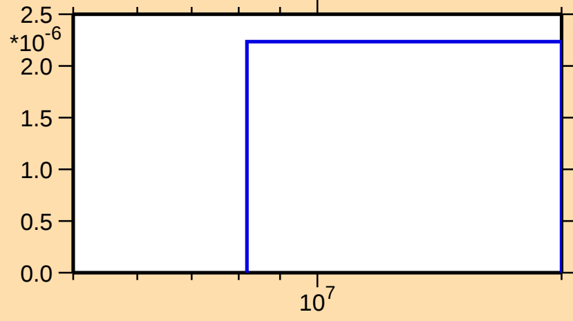
\sigma vs. E for ^{168}\text{Re}(n,\text{nd})
