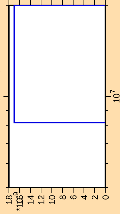
\Delta\sigma/\sigma vs. E for ^{168}\text{Re}(\text{mt 11})
