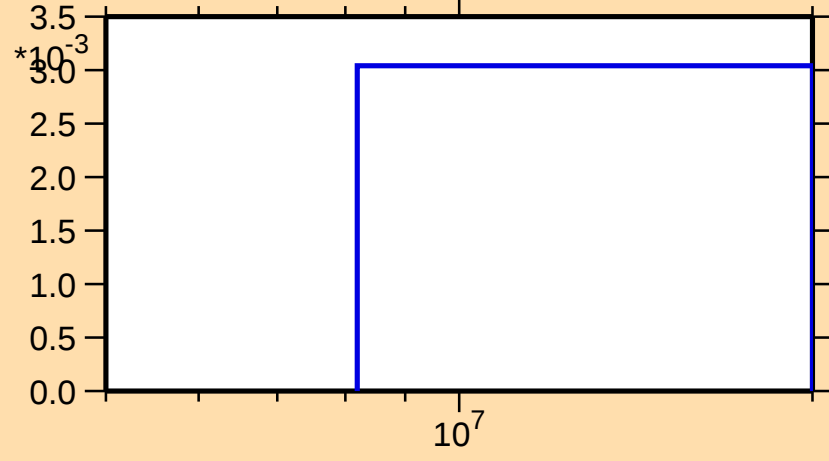
\sigma vs. E for ^{168}\text{Re}(n,2np)
