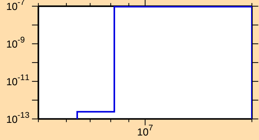
\sigma vs. E for ^{168}\text{Re}(\text{mt117})
