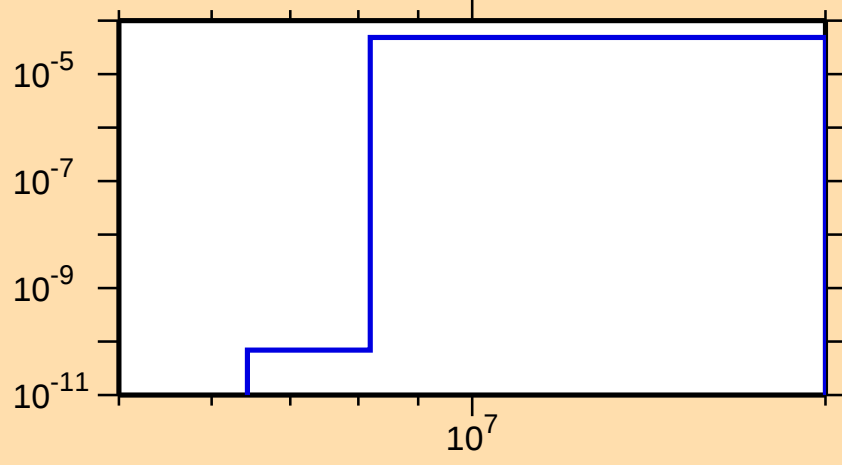
\sigma vs. E for ^{168}\text{Re}(\text{mt } 45)
