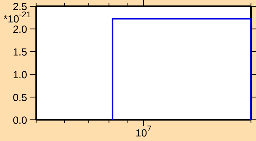
\sigma vs. E for ^{168}\text{Re}(\text{mt 11})
