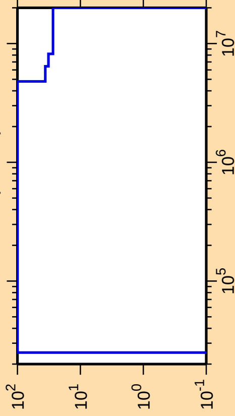
\Delta\sigma/\sigma vs. E for ^{168}\text{Re}(n,\text{inel.})
