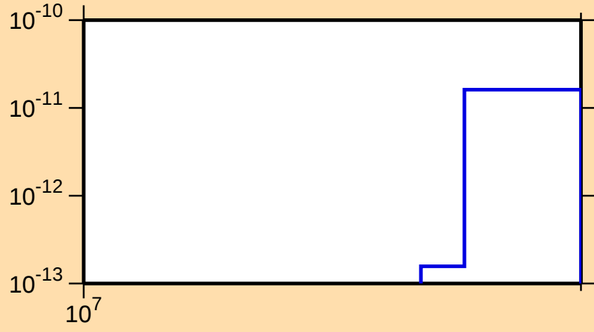
\sigma vs. E for ^{173}\text{Re}(\text{mt } 34)
