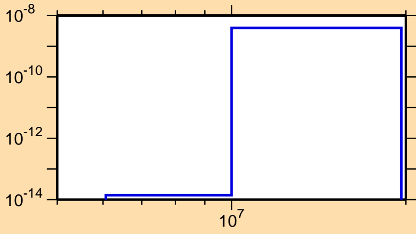
\sigma vs. E for ^{173}\text{Re}(\text{mt117})
