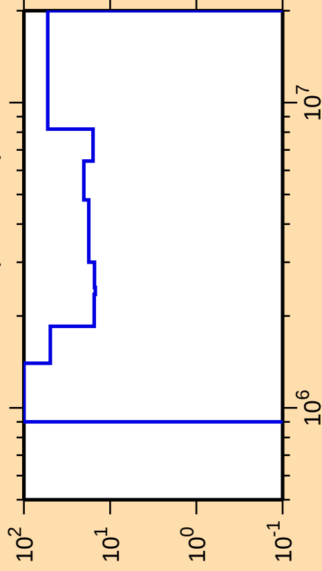
\Delta\sigma/\sigma vs. E for ^{173}\text{Re}(n,n_{\text{cont}}) .
