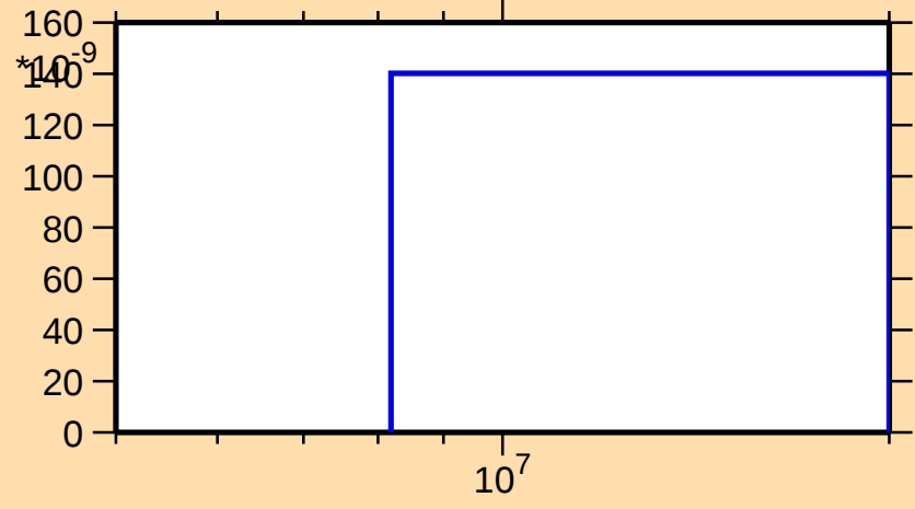
\sigma vs. E for ^{173}\text{Re}(n,2n\alpha)
