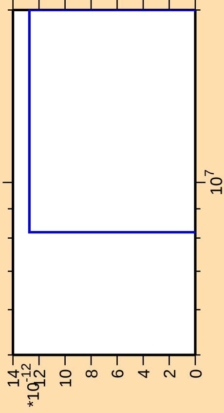
\Delta\sigma/\sigma vs. E for ^{173}\text{Re}(\text{mt } 42)
