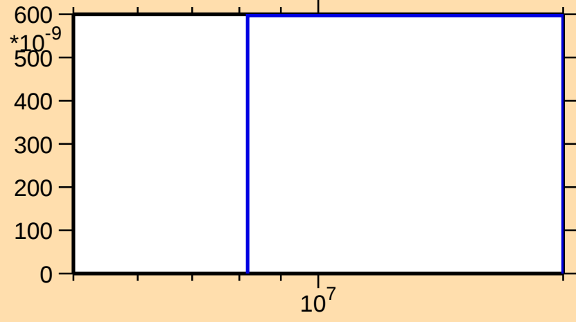
\sigma vs. E for ^{173}\text{Re}(\text{mt } 45)
