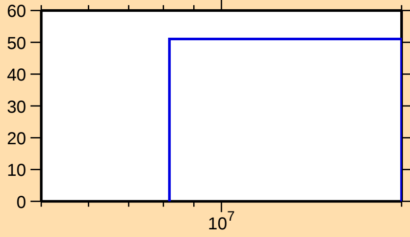
\Delta\sigma/\sigma vs. E for ^{173}\text{Re}(n,\text{inel.})
