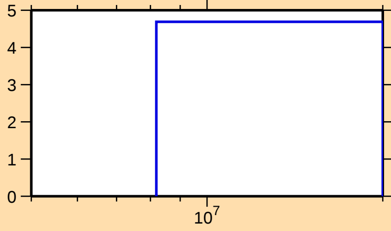
\Delta\sigma/\sigma vs. E for ^{173}\text{Re}(n,\text{tot.})
