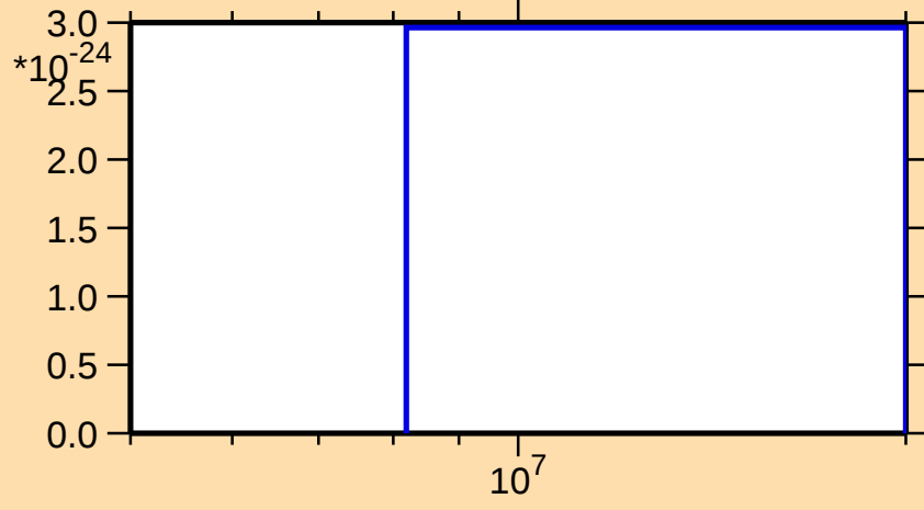
\sigma vs. E for ^{173}\text{Re}(\text{mt } 42)
