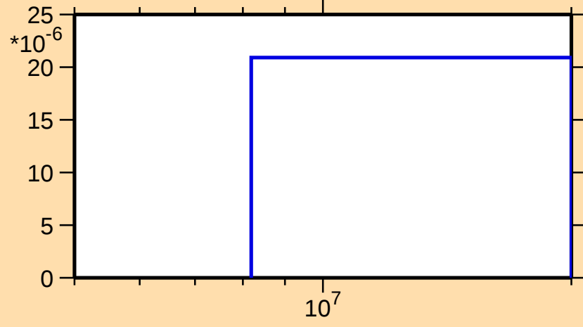
\sigma vs. E for ^{173}\text{Re}(n,2np)
