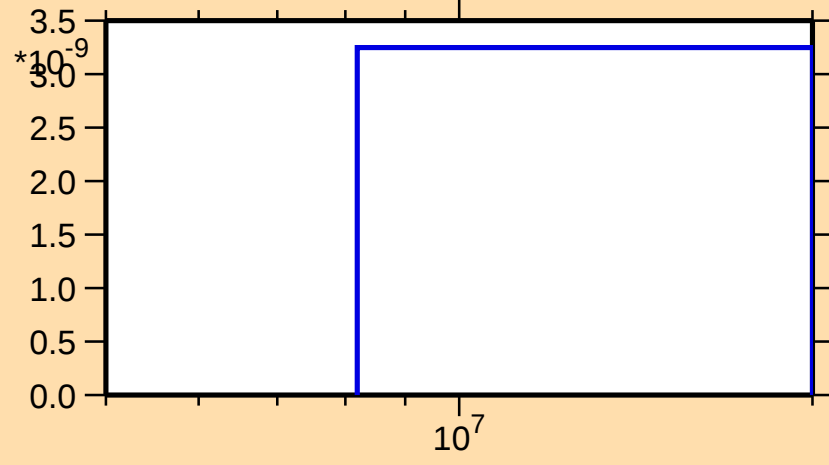
\sigma vs. E for ^{173}\text{Re}(n,\text{pd})
