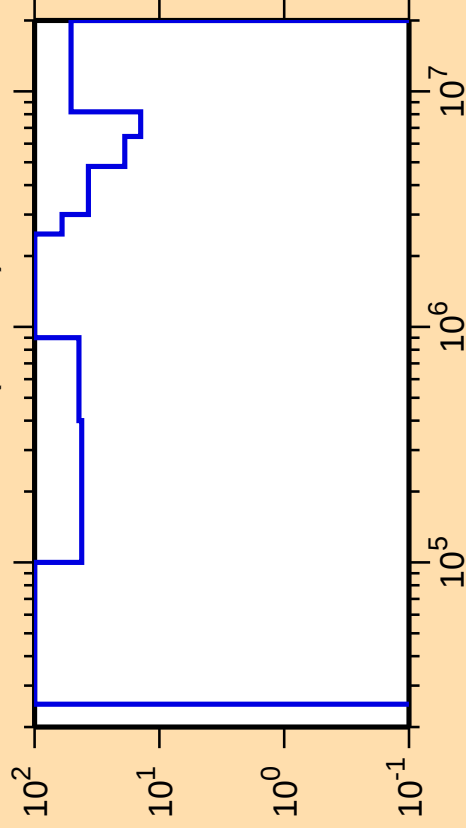
\Delta\sigma/\sigma vs. E for ^{173}\text{Re}(n,\text{inel.})
