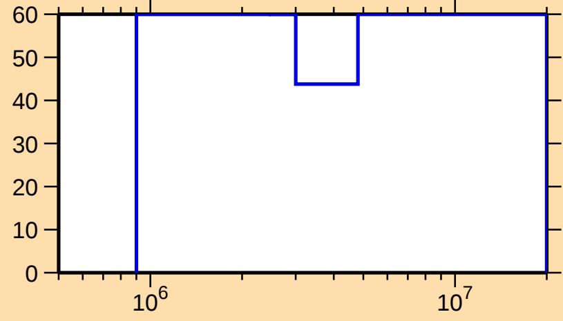
\Delta\sigma/\sigma vs. E for ^{173}\text{Re}(n,n_1)
