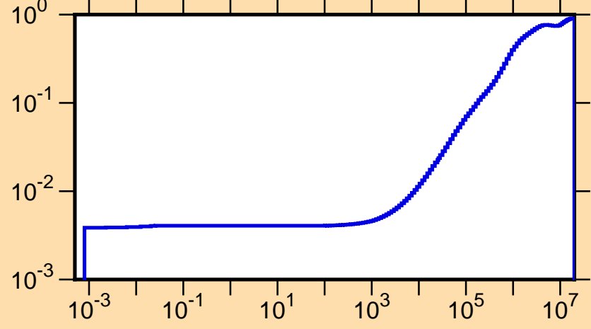
\mu vs. E for ^{175}\text{Re}(\text{mt251})
