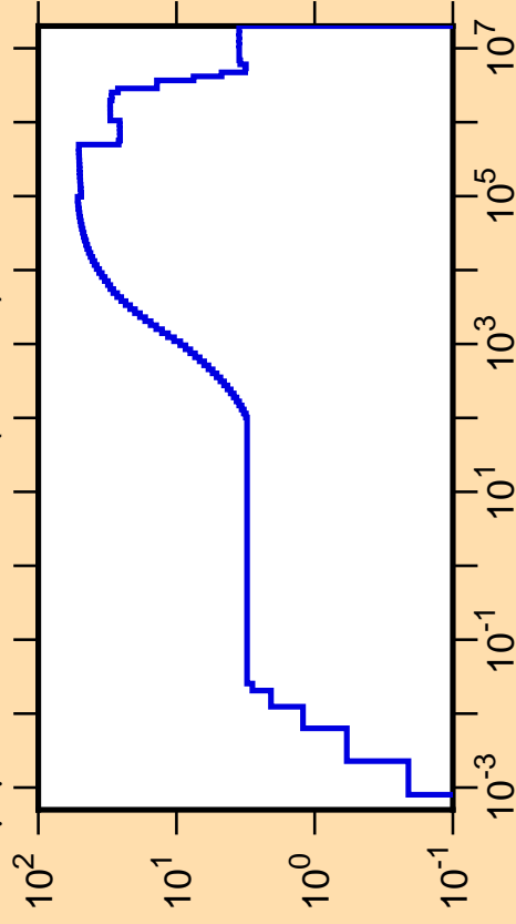
\Delta\mu/\mu vs. E for ^{175}\text{Re}(\text{mt251})
