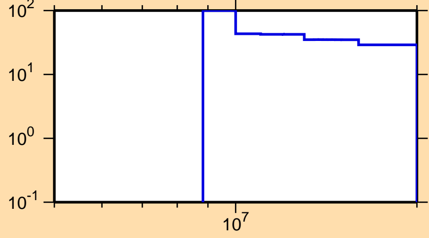
\Delta\sigma/\sigma vs. E for ^{175}\text{Re}(n,2n)
