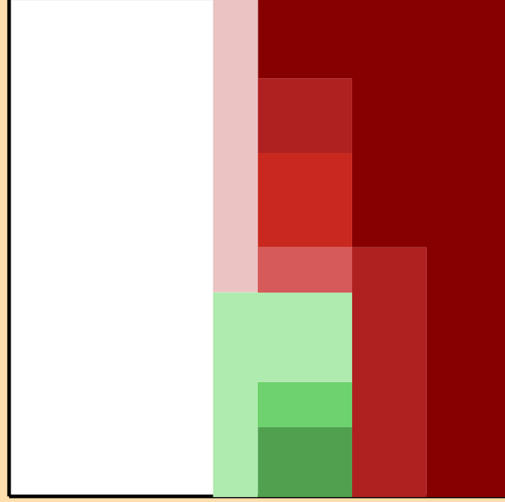
\Delta\sigma/\sigma vs. E for ^{175}\text{Re}(n,2n)
