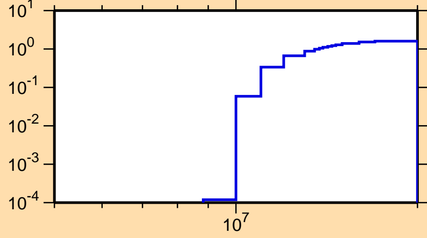
\sigma vs. E for ^{175}\text{Re}(n,2n)
