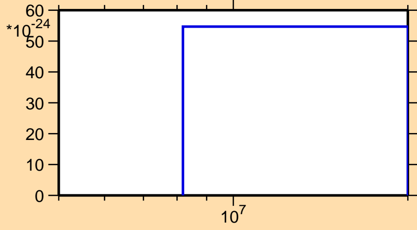
\sigma vs. E for ^{175}\text{Re}(\text{mt } 42)
