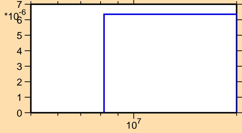
\sigma vs. E for ^{175}\text{Re}(n,2np)
