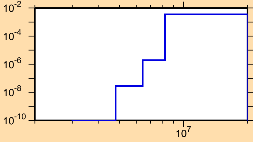
\sigma vs. E for ^{175}\text{Re}(n,d)
