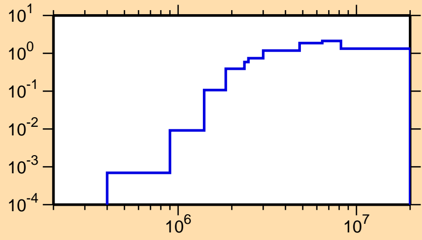
\sigma vs. E for ^{175}\text{Re}(n,n\text{cont.})
