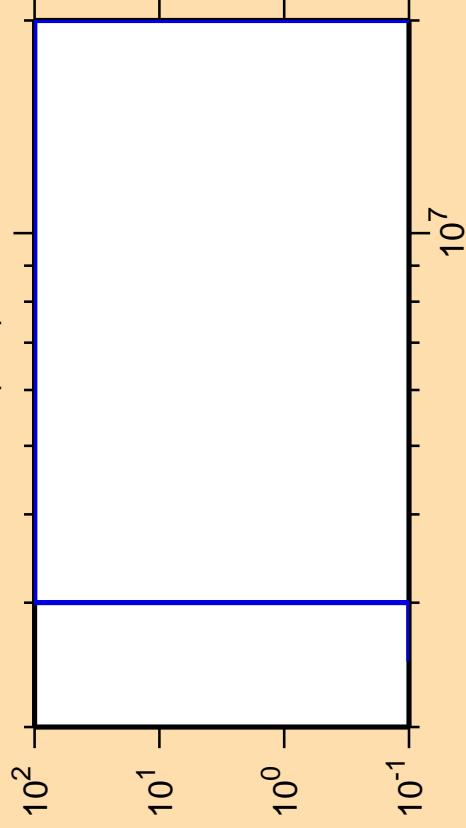
\Delta\sigma/\sigma vs. E for ^{175}\text{Re}(n,d)
