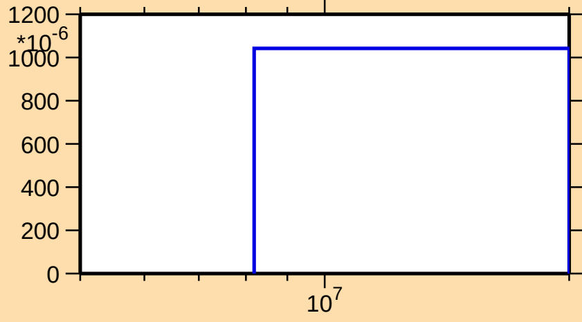
\sigma vs. E for ^{181}\text{Re}(n,3n)
