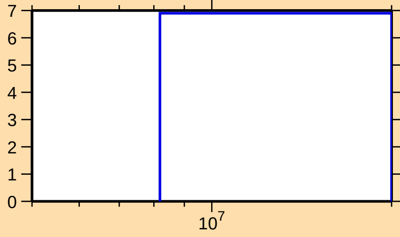
\Delta\sigma/\sigma vs. E for ^{181}\text{Re}(n,\text{el.})
