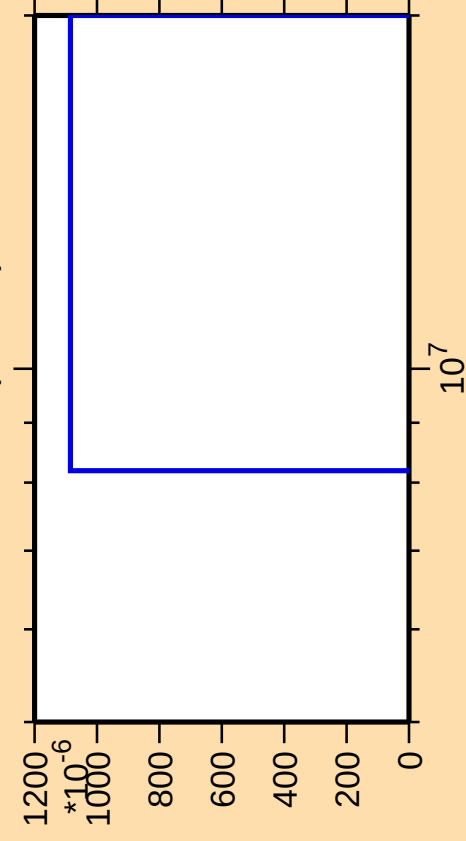
\Delta\sigma/\sigma vs. E for ^{181}\text{Re}(n,3n\alpha)
