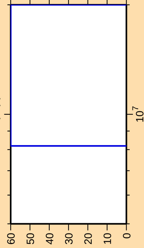
\Delta\sigma/\sigma vs. E for ^{181}\text{Re}(n,p)
