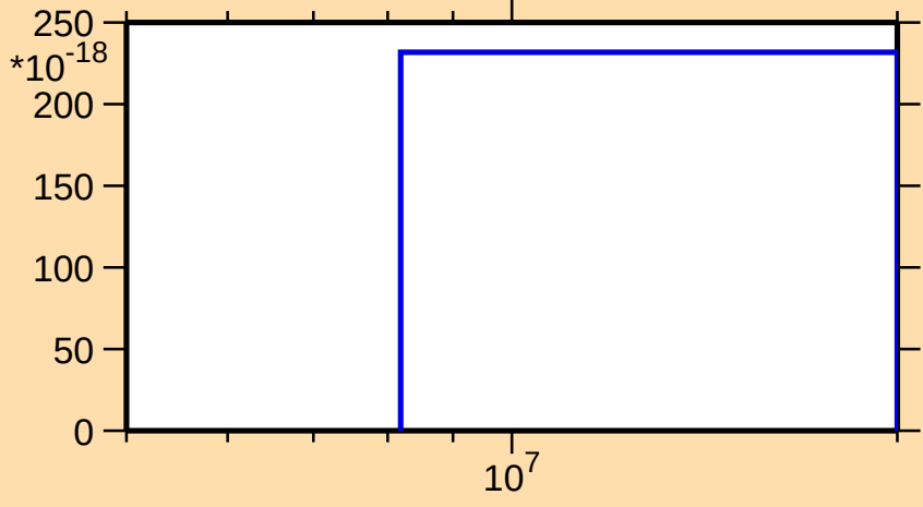
\sigma vs. E for ^{181}\text{Re}(n,3n\alpha)
