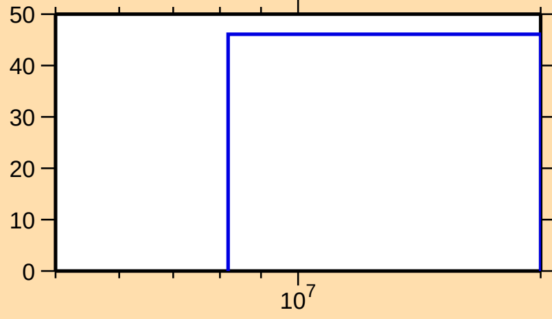
\Delta\sigma/\sigma vs. E for ^{181}\text{Re}(n,\text{inel.})
