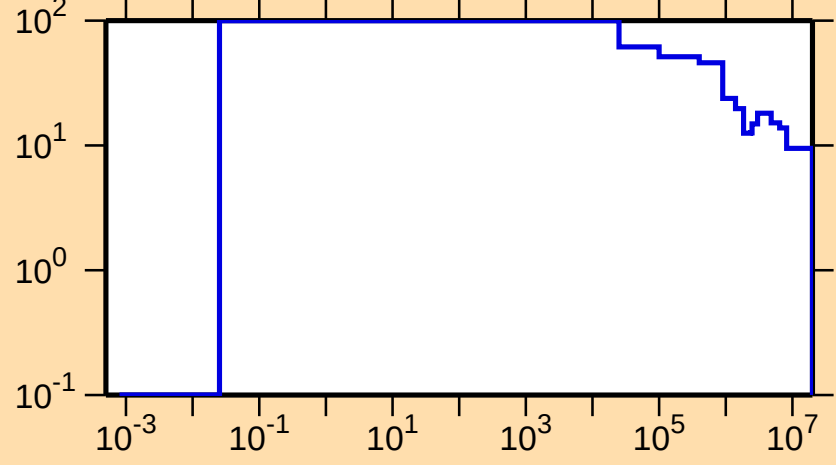
\Delta\sigma/\sigma vs. E for ^{181}\text{Re}(n,\text{nonel.})
