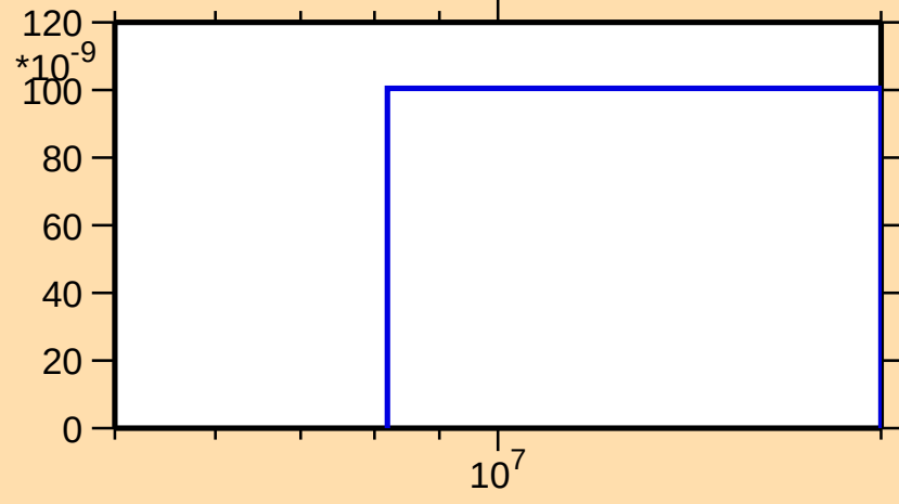
\sigma vs. E for ^{181}\text{Re}(n,2np)
