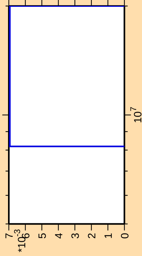
\Delta\sigma/\sigma vs. E for ^{181}\text{Re}(n,\text{pd})
