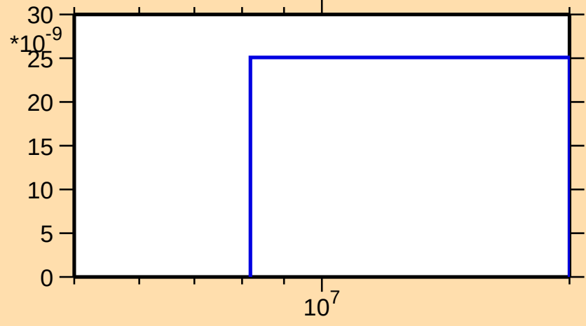
\sigma vs. E for ^{181}\text{Re}(n,2n\alpha)
