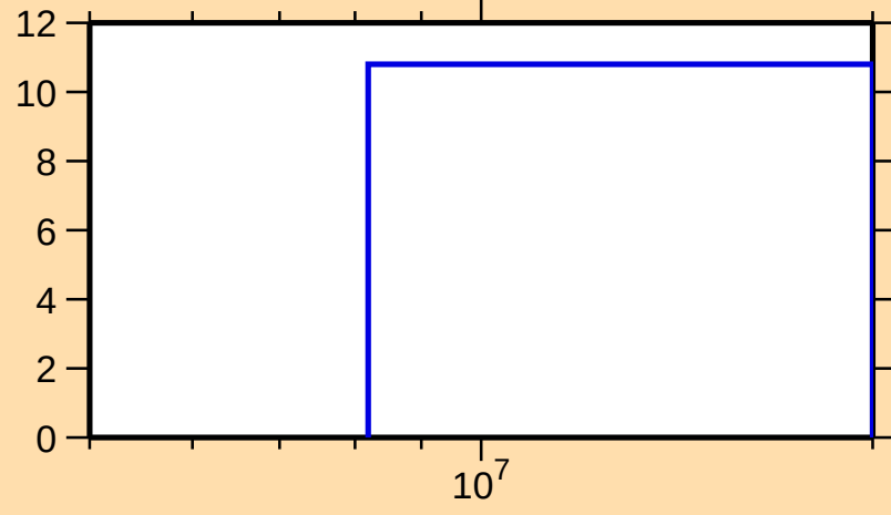
\Delta\sigma/\sigma vs. E for ^{181}\text{Re}(n,2n)
