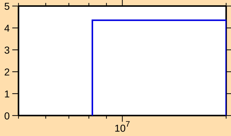
\Delta\sigma/\sigma vs. E for ^{181}\text{Re}(n,\text{tot.})
