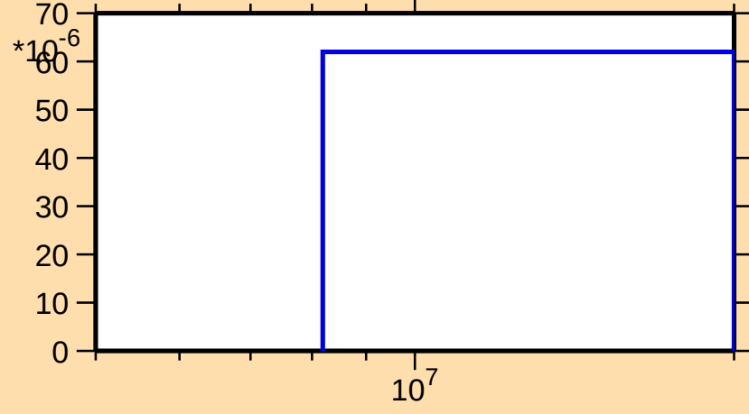
\sigma vs. E for ^{181}\text{Re}(n,t)
