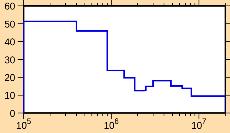
\Delta\sigma/\sigma vs. E for ^{181}\text{Re}(n,\text{nonel.})
