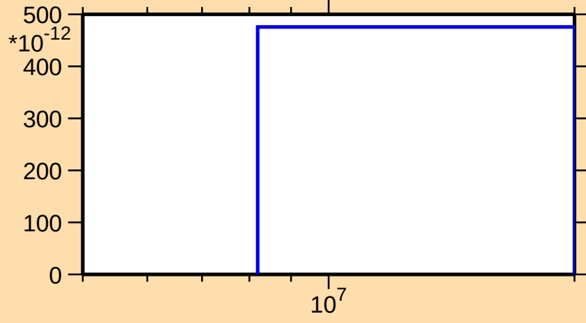
\sigma vs. E for ^{181}\text{Re}(n,\text{He3})
