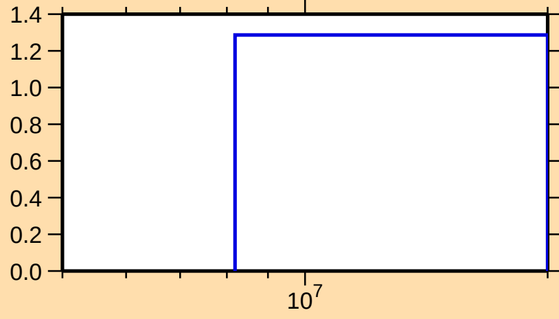
\sigma vs. E for ^{181}\text{Re}(n,2n)
