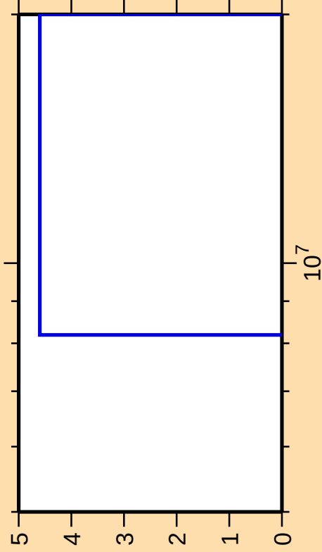
\Delta\sigma/\sigma vs. E for ^{181}\text{Re}(\text{mt } 45)
