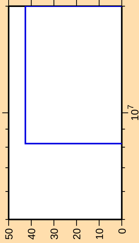
\Delta\sigma/\sigma vs. E for ^{181}\text{Re}(n,n\text{cont.})
