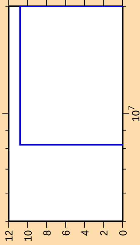
\Delta\sigma/\sigma vs. E for ^{181}\text{Re}(n,2n)
