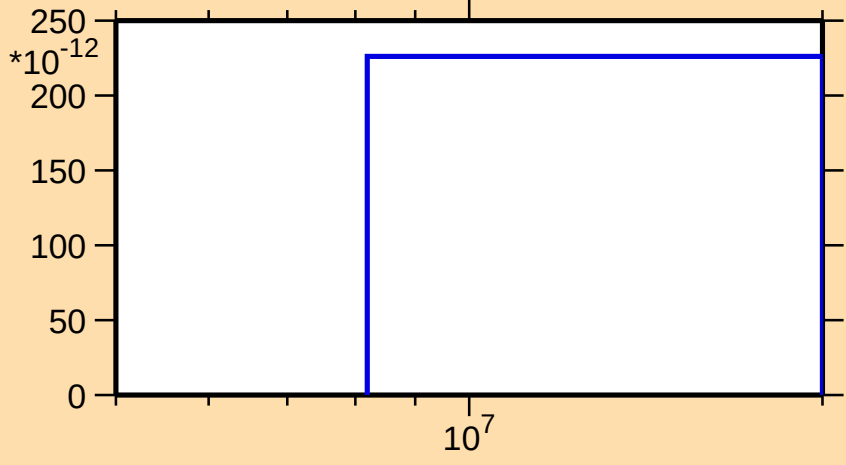
\sigma vs. E for ^{181}\text{Re}(n,p\alpha)
