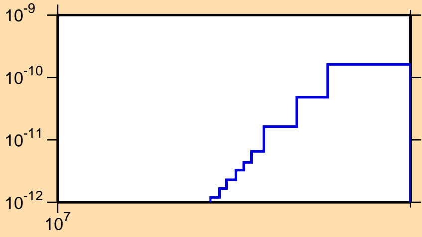
\sigma vs. E for ^{183}\text{Re}(n,p\alpha)
