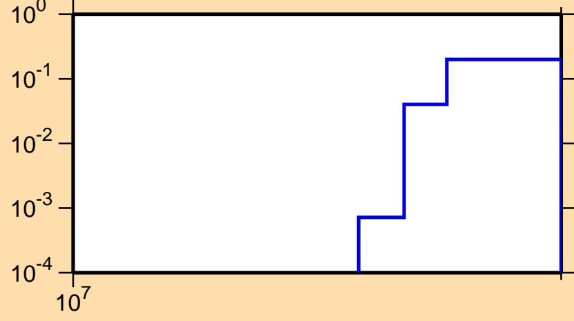
\sigma vs. E for ^{183}\text{Re}(n,3n)
