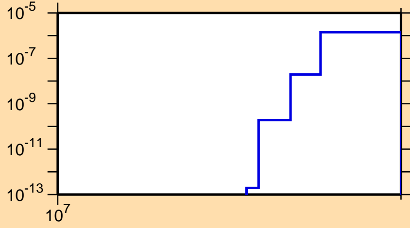
\sigma vs. E for ^{183}\text{Re}(n,2np)
