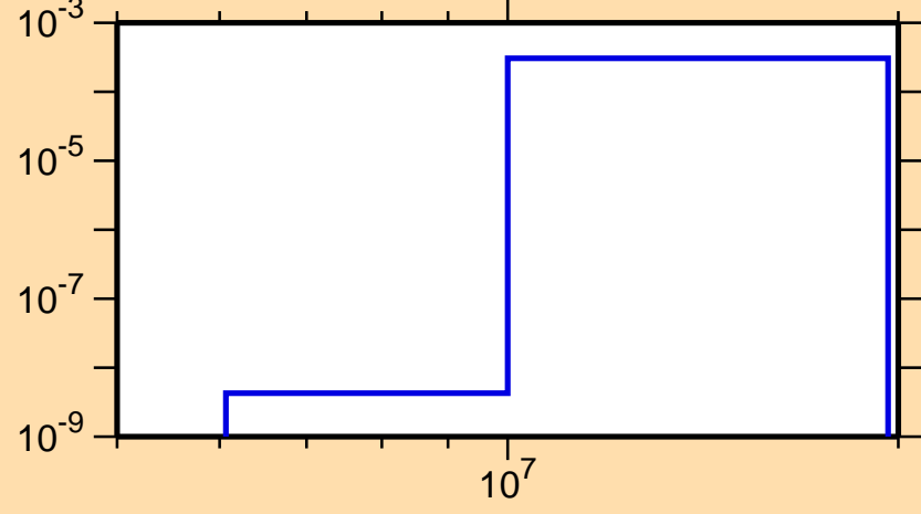
\sigma vs. E for ^{185}\text{Re}(n,np)
