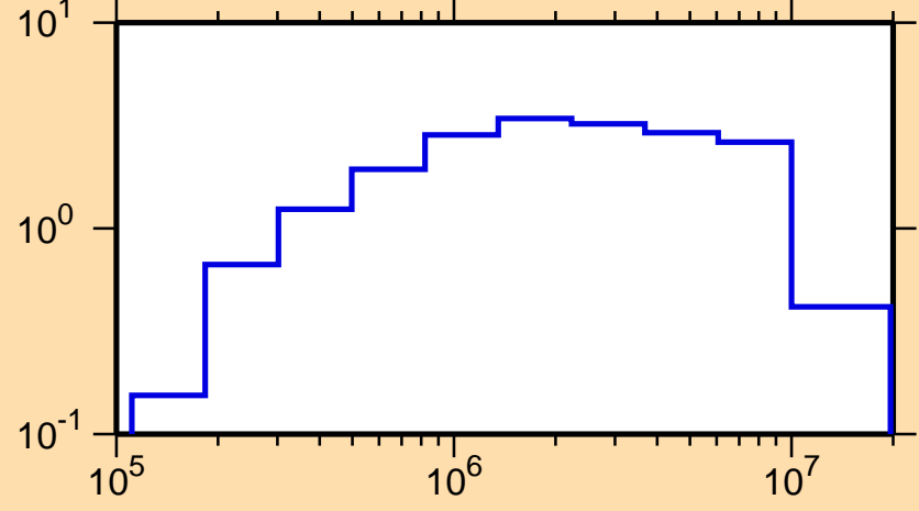
\sigma vs. E for ^{185}\text{Re}(n,\text{inel.})
