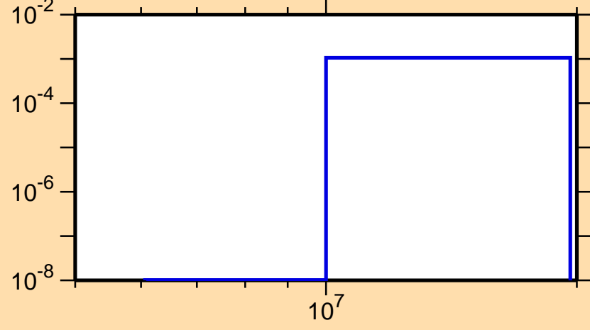
\sigma vs. E for ^{185}\text{Re}(n,d)
