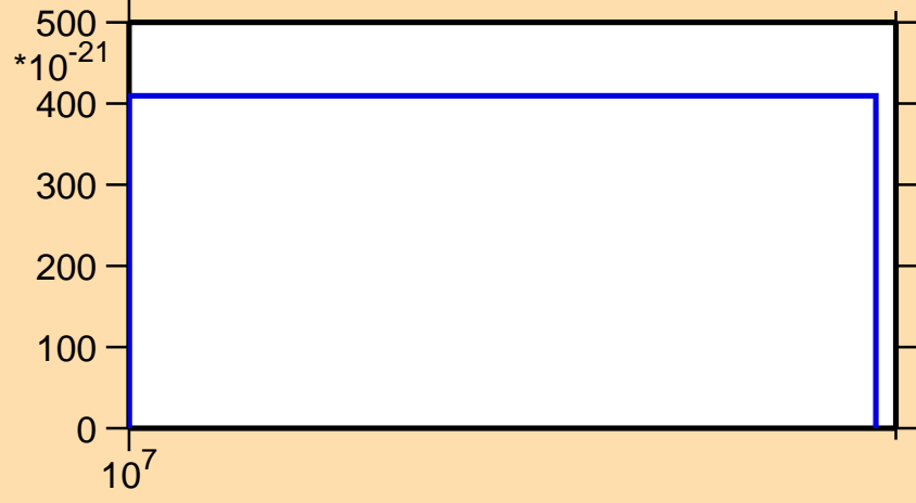
\sigma vs. E for ^{185}\text{Re}(\text{mt } 42)
