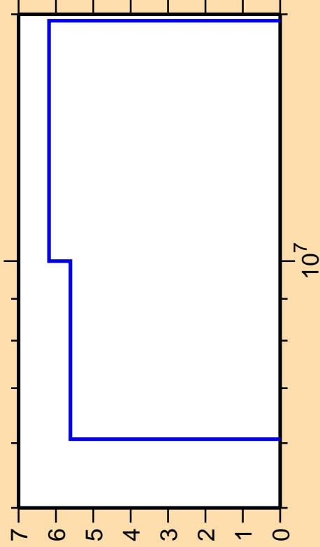
\Delta\sigma/\sigma vs. E for ^{185}\text{Re}(n,2n)
