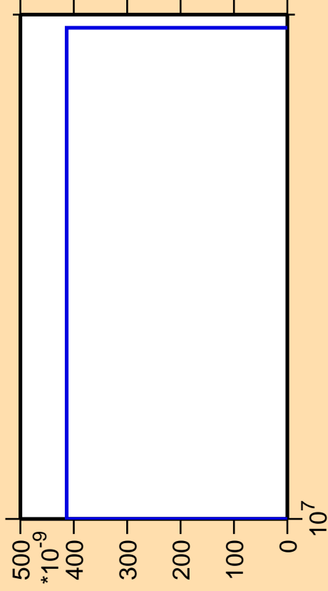
\Delta\sigma/\sigma vs. E for ^{185}\text{Re}(\text{mt } 42)
