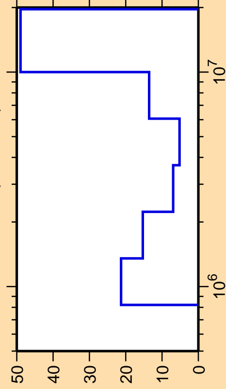
\Delta\sigma/\sigma vs. E for ^{185}\text{Re}(n,\text{ncont.})
