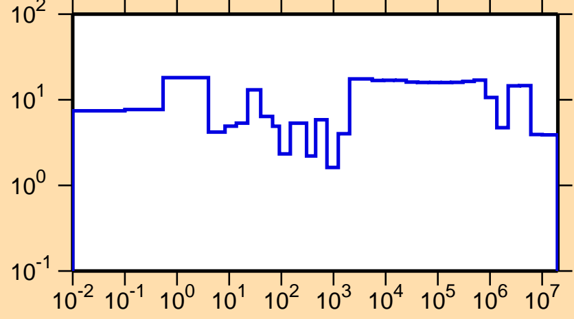
\Delta\sigma/\sigma vs. E for ^{185}\text{Re}(n,\text{el.})
