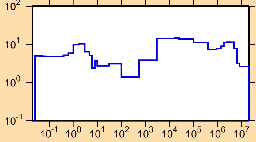
\Delta\sigma/\sigma vs. E for ^{185}\text{Re}(n,\text{tot.})
