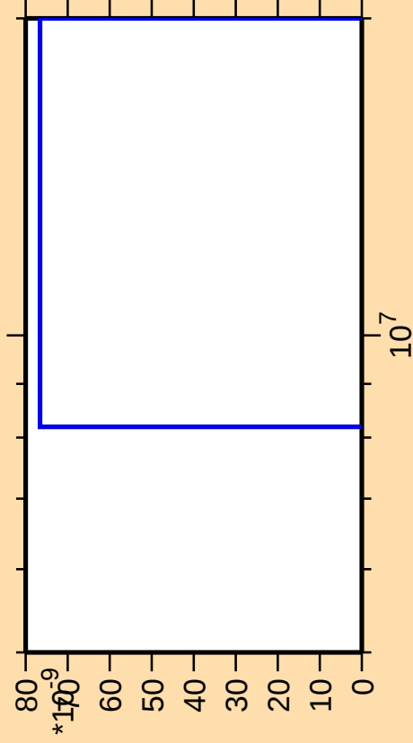
\Delta\sigma/\sigma vs. E for ^{95}\text{Rh}(n,nt)
