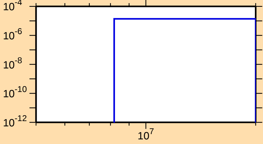
\sigma vs. E for ^{95}\text{Rh}(n,t)
