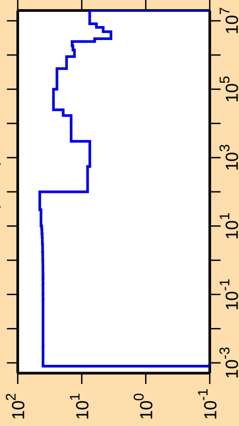
\Delta\sigma/\sigma vs. E for ^{95}\text{Rh}(n,\text{el.})
