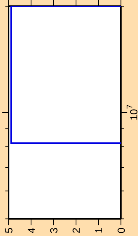
\Delta\sigma/\sigma vs. E for ^{95}\text{Rh}(\text{mt117})
