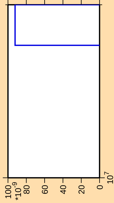
\Delta\sigma/\sigma vs. E for ^{95}\text{Rh}(n,\text{nt})
