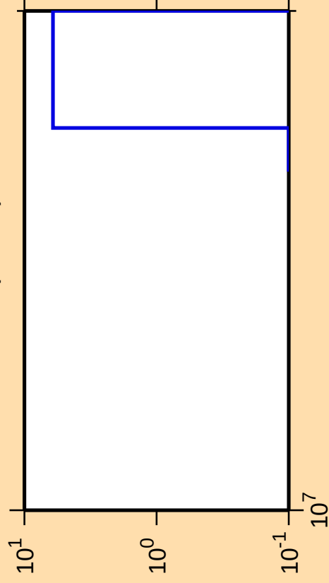
\Delta\sigma/\sigma vs. E for ^{95}\text{Rh}(\text{mt } 34)
