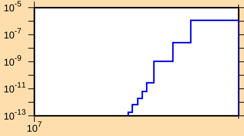
\sigma vs. E for ^{95}\text{Rh}(\text{mt } 45)
