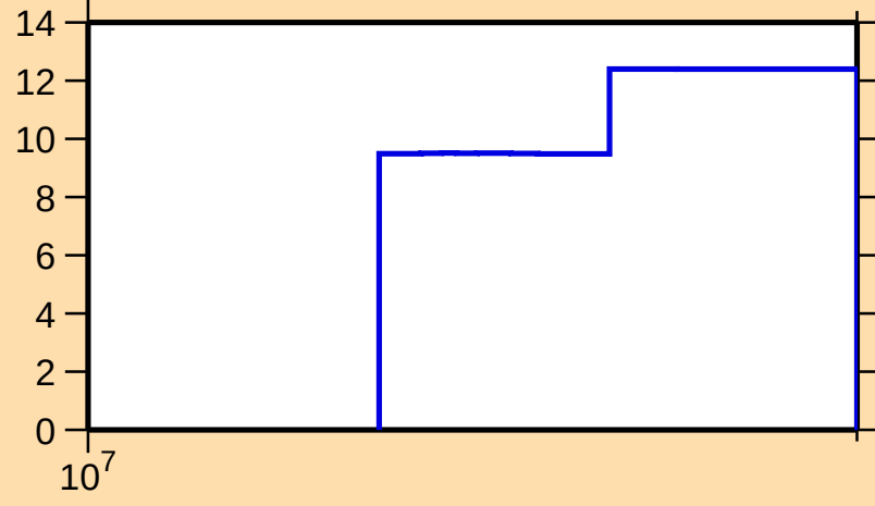
\Delta\sigma/\sigma vs. E for ^{95}\text{Rh}(n,\text{el.})
