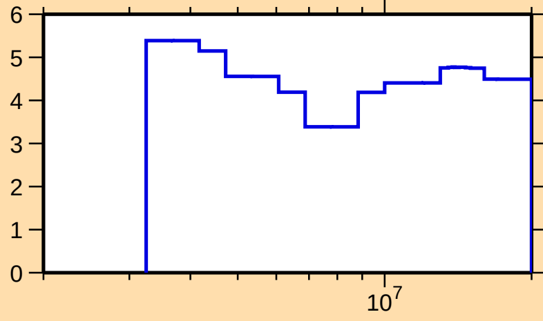
\Delta\sigma/\sigma vs. E for ^{95}\text{Rh}(n,n\text{onel.})
