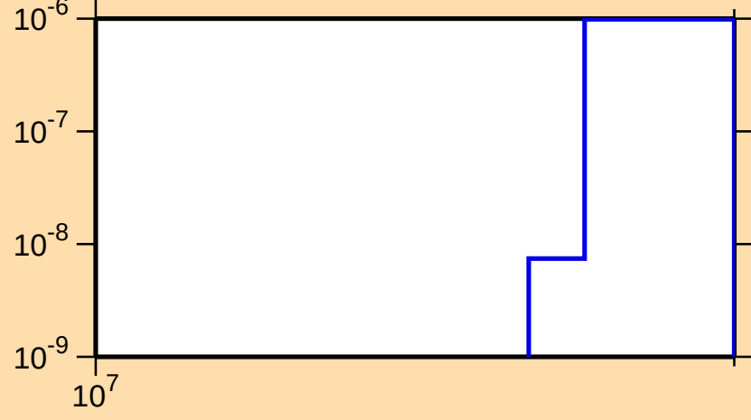
\sigma vs. E for ^{95}\text{Rh}(n,\text{nd})
