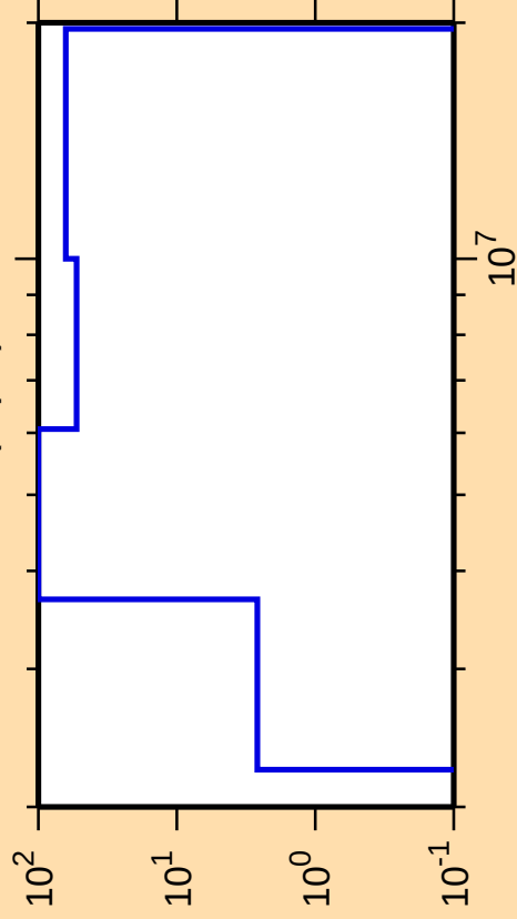
\Delta\sigma/\sigma vs. E for ^{95}\text{Rh}(n,p\alpha)
