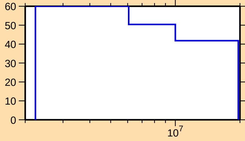
\Delta\sigma/\sigma vs. E for ^{95}\text{Rh}(n,n\text{cont.})
