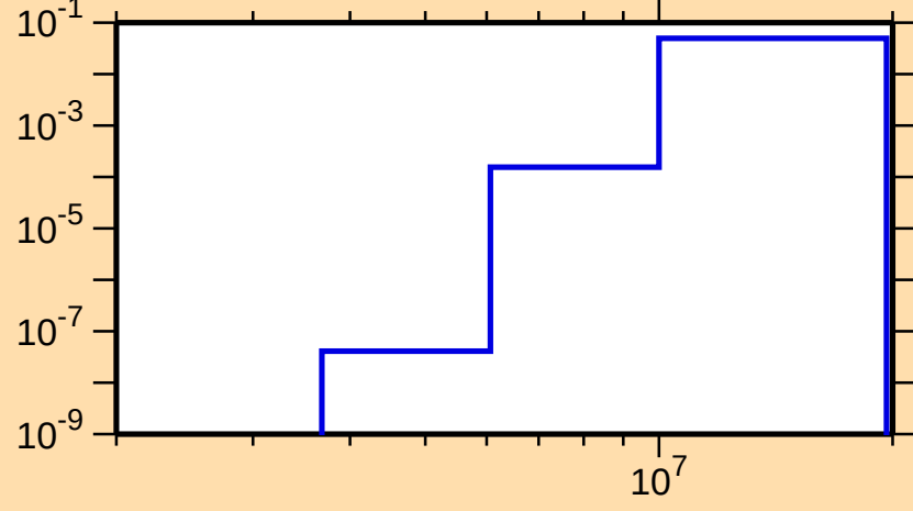
\sigma vs. E for ^{95}\text{Rh}(n,p\alpha)
