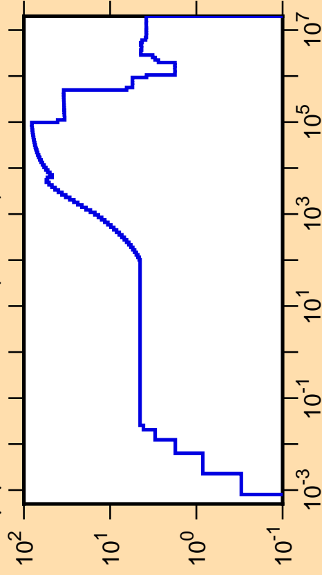
\Delta\mu/\mu vs. E for ^{96}\text{Rh}(\text{mt251})
